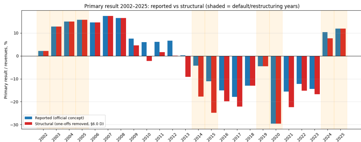
Figure 7: Official versus structural primary result: one-off and accounting-driven revenues removed.
