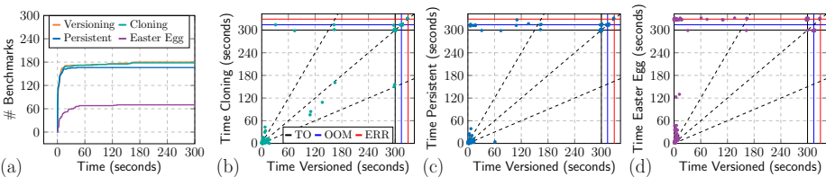
Figure 1: Run time Comparison of TheSy.
