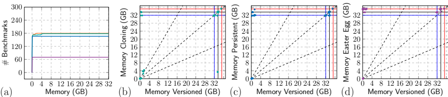
Figure 2: Memory Comparison of TheSy.
