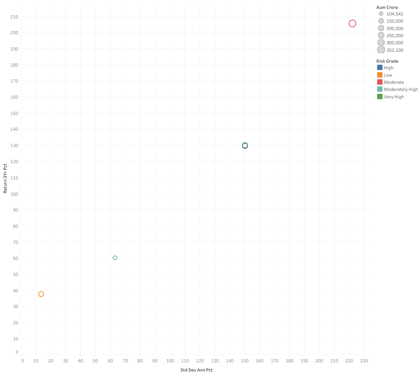
Risk vs Return
