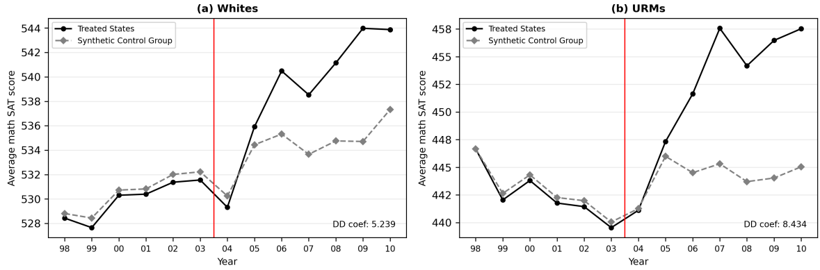
Figure 2: Replication of Figure 3: Synthetic Control Estimates of the Effect of AA on SAT Math Scores. Left panel: whites. Right panel: URM (Black and Hispanic). Treated unit = Texas (TX + LA + MS combined). Vertical red line marks 2003.5 (treatment). DD coef labels show mean post-gap minus mean pre-gap.
