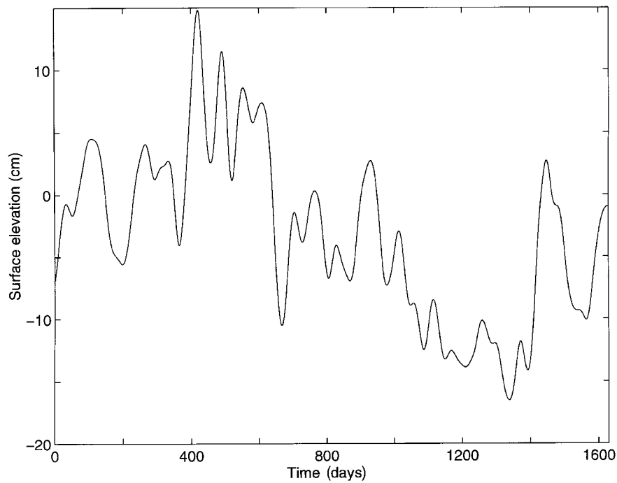
Figure 72. Altimeter data over the equatorial sea at 174° E on the Equator. The starting date of the data was 1 April 1985.
