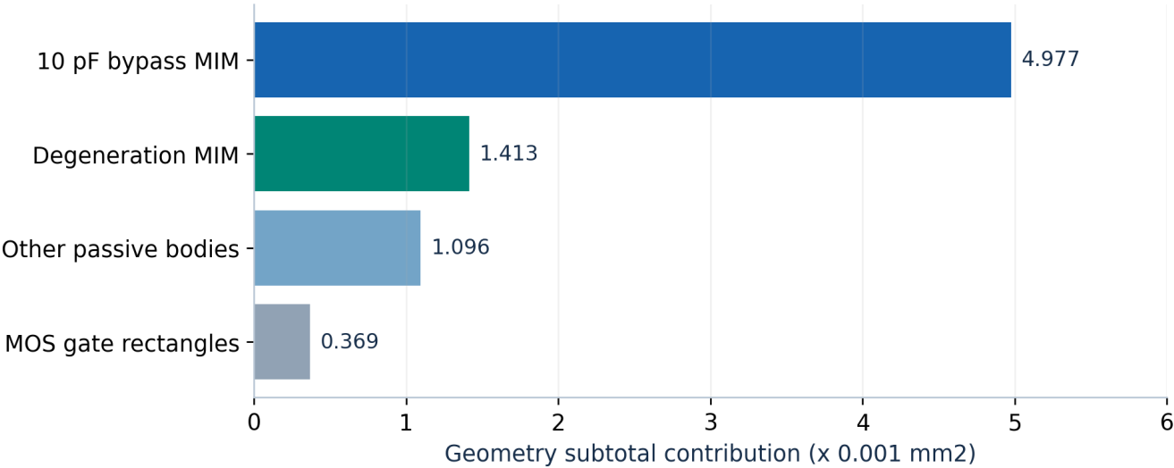
Figure 12. Netlist-derived geometry inventory for all 27 physical instances. Values count passive bodies/plates and MOS W x L rectangles, with instance multiplicity; they are not a routed floorplan.
