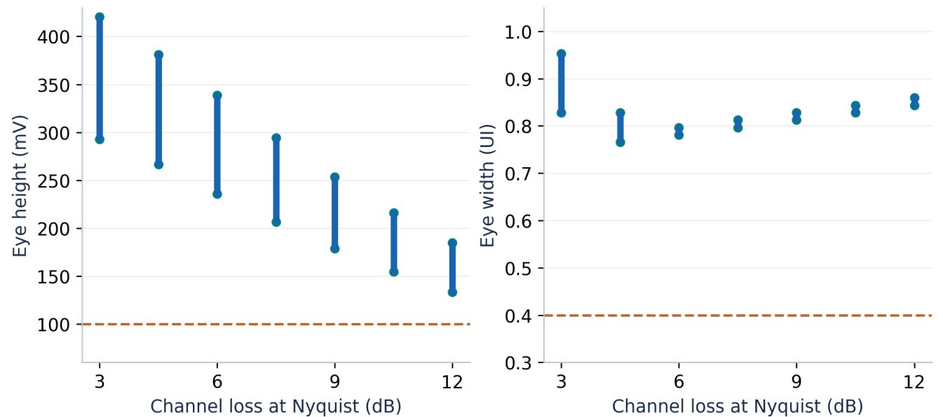
Figure 9. Minimum-to-maximum modelled eye over the 45 PVT points at each constructed channel loss, with ideal behavioural 1-tap DFE. Dashed lines: 100 mV and 0.4 UI thresholds.
