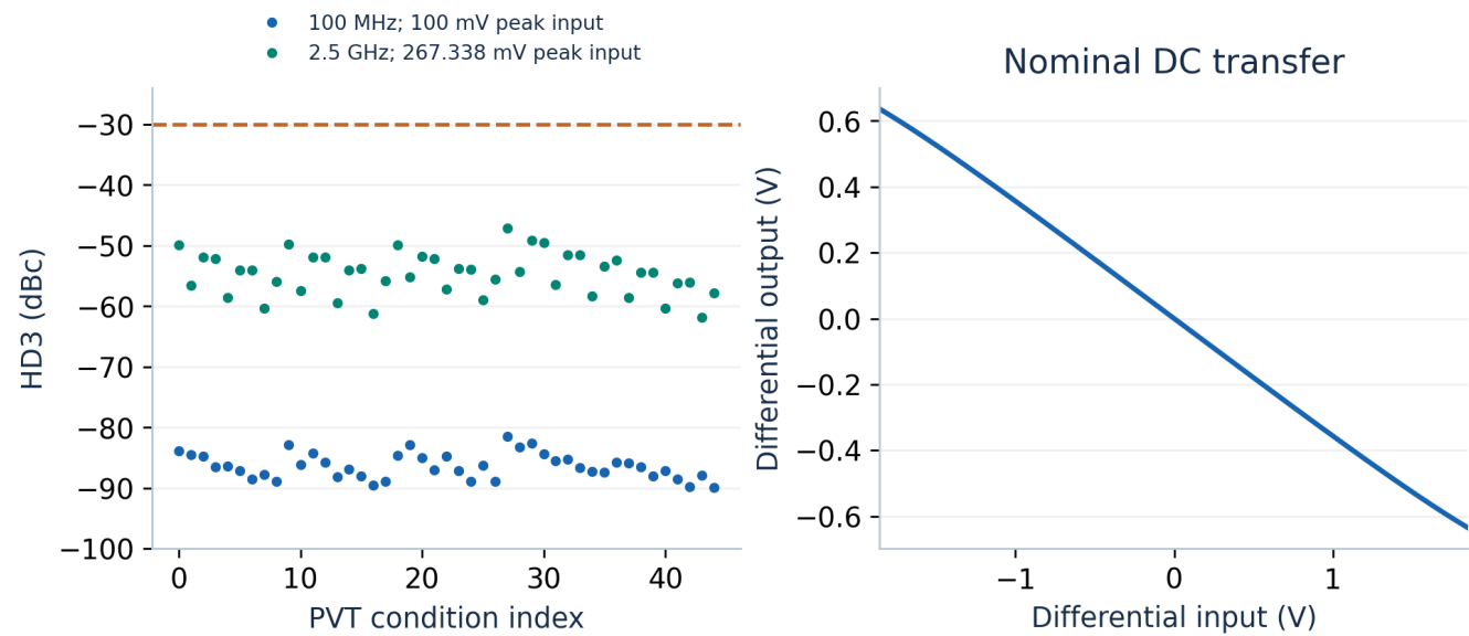
Figure 8. HD3 at two separately tested tone frequencies across PVT (left) and the raw nominal DC transfer (right). Input amplitudes are differential peak values, not peak-to-peak.
