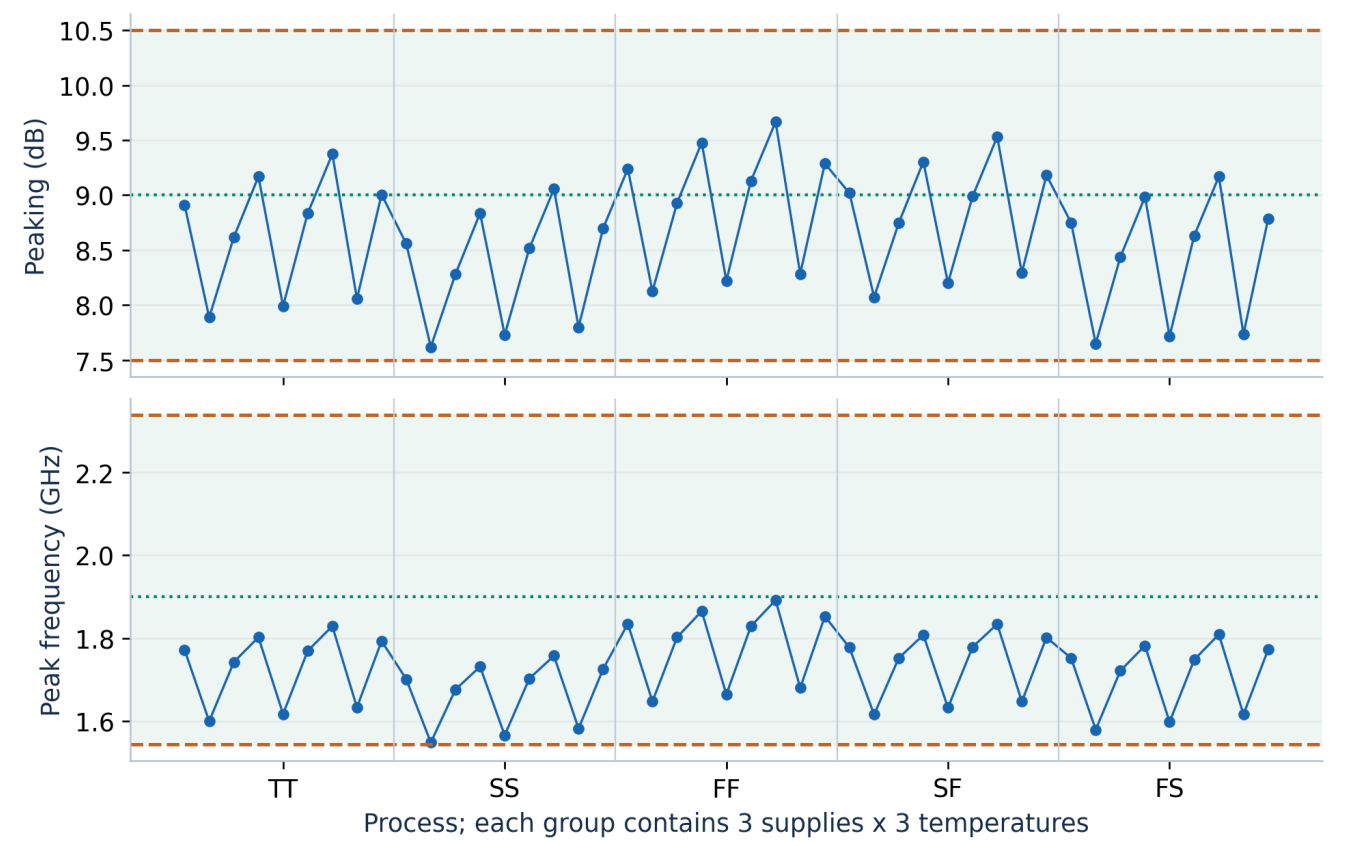
Figure 6. All 45 measured points. Shading and dashed lines mark project request-matching bands; dotted lines mark the requested centres. Point order within each process is supply/temperature order.
