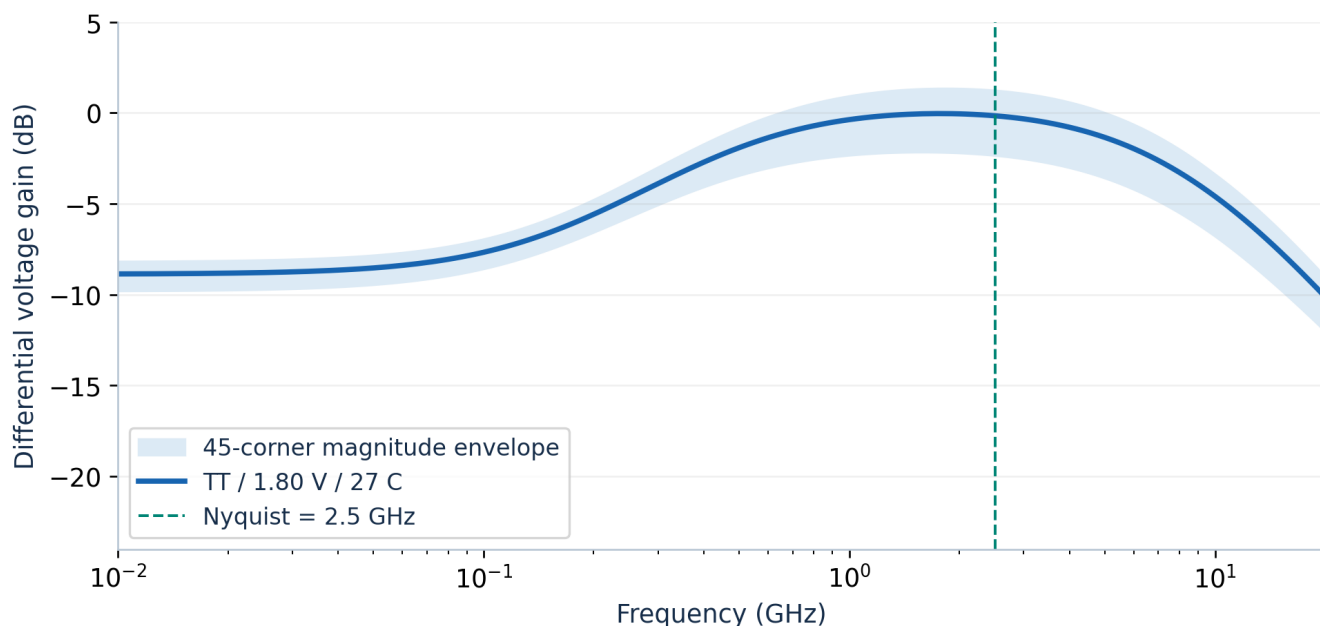
Figure 5. Raw SPICE AC magnitude: final nominal peaking 8.834 dB at 1.769 GHz; shaded limits show the 45-corner envelope. The curve is absolute voltage gain, not gain normalised to 0 dB.
