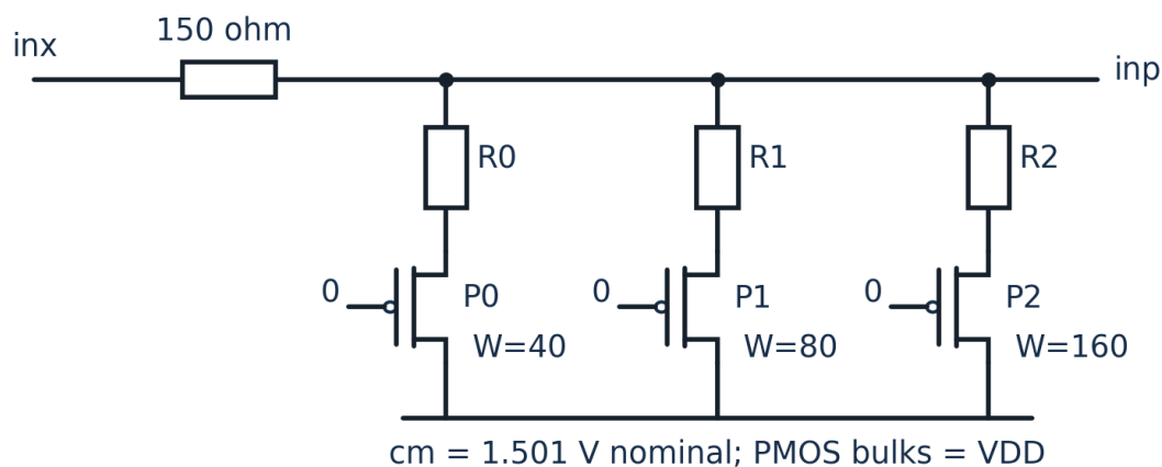
Figure 4. Positive input leg; the negative leg is identical. Three PMOS-switched shunt branches join inp to cm . A7 holds all three gates at 0 V (ON). W labels are total microns; L = 0.15 \mu m .
