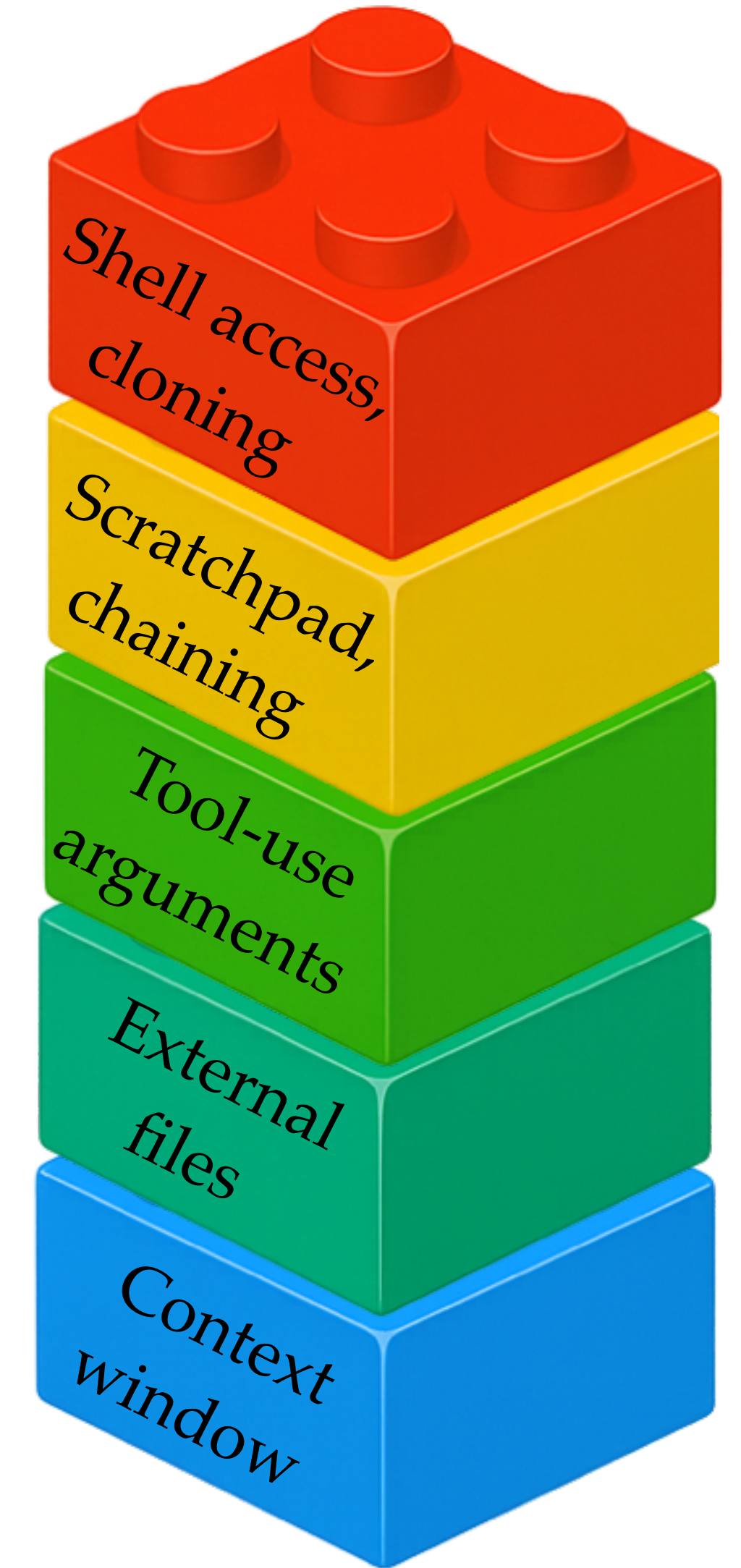
Attack surfaces
