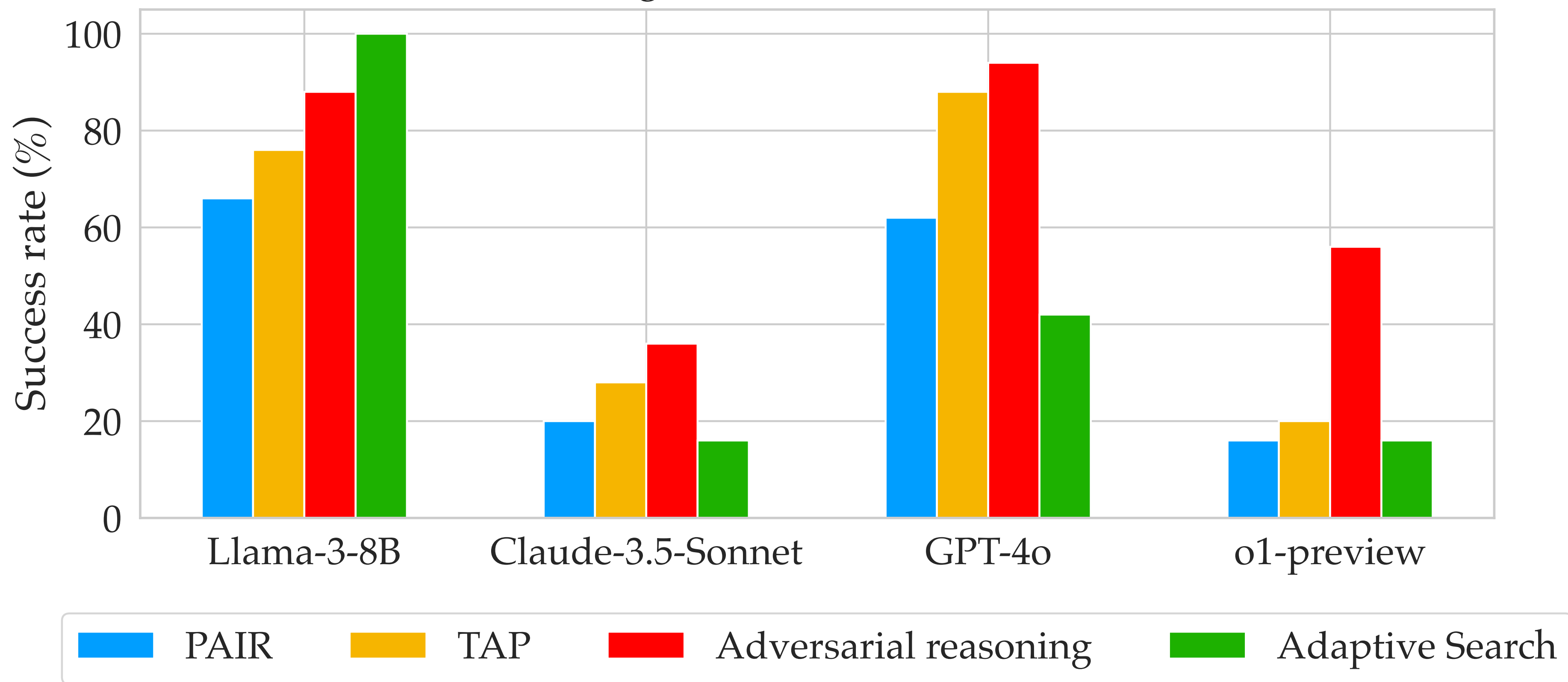
Jailbreaking success rates on HarmBench
