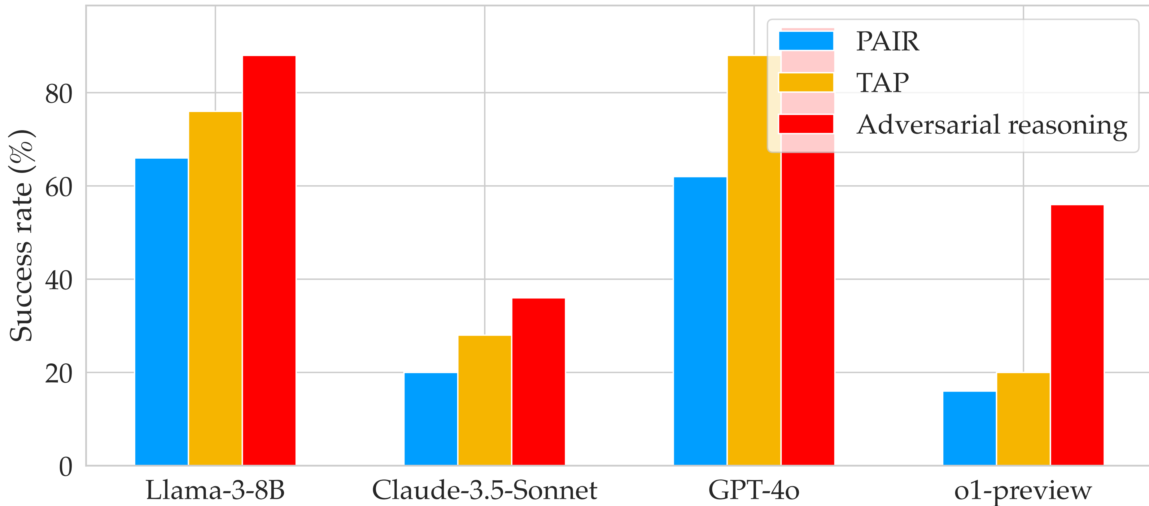
Jailbreaking success rates on HarmBench
