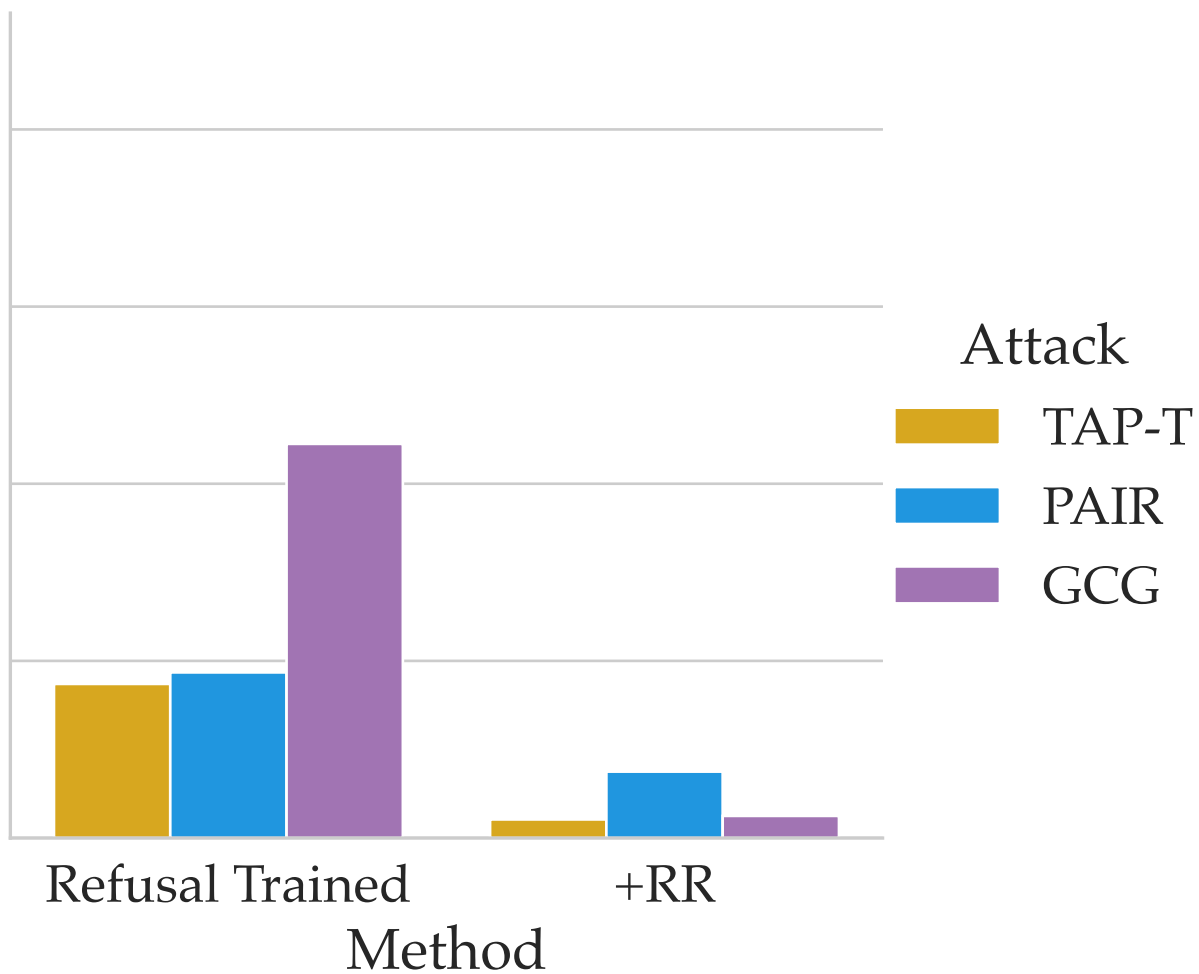
Llama-3-8B-Instruct
