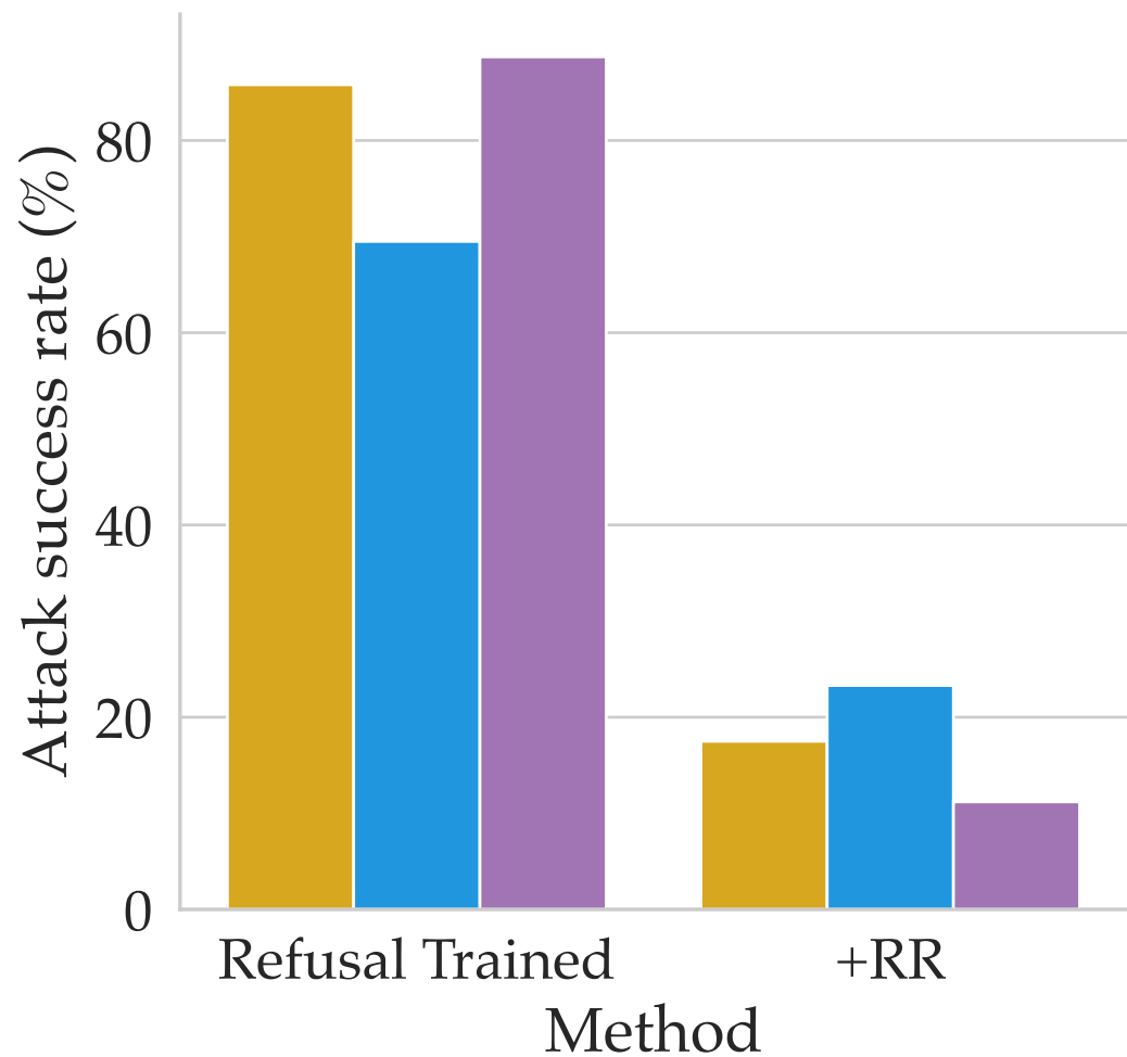
Mistral-7B-Instruct-v2
