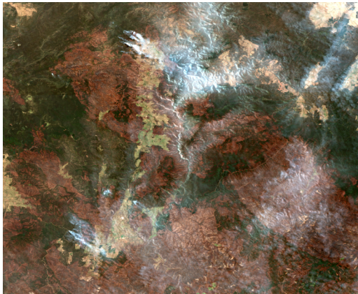
RGB image
