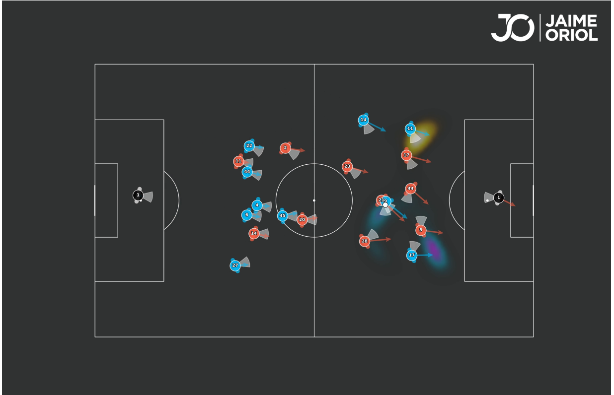
Figure 6: Diagonal Opportunity Surface. For every cell, DOS is the extra attacker pitch control bought by the best diagonal delivery over the best orthogonal one, given the defenders’ real orientation and what they can see. Rendered through the scanning gate (Sec. 6.4): cyan-to-magenta marks diagonal opportunity the on-ball player currently sees or has recently scanned; amber marks opportunity ahead of him that he is no longer watching. Same frame as Figs. 4 and 5. Video: DOS_Video.mp4 .
