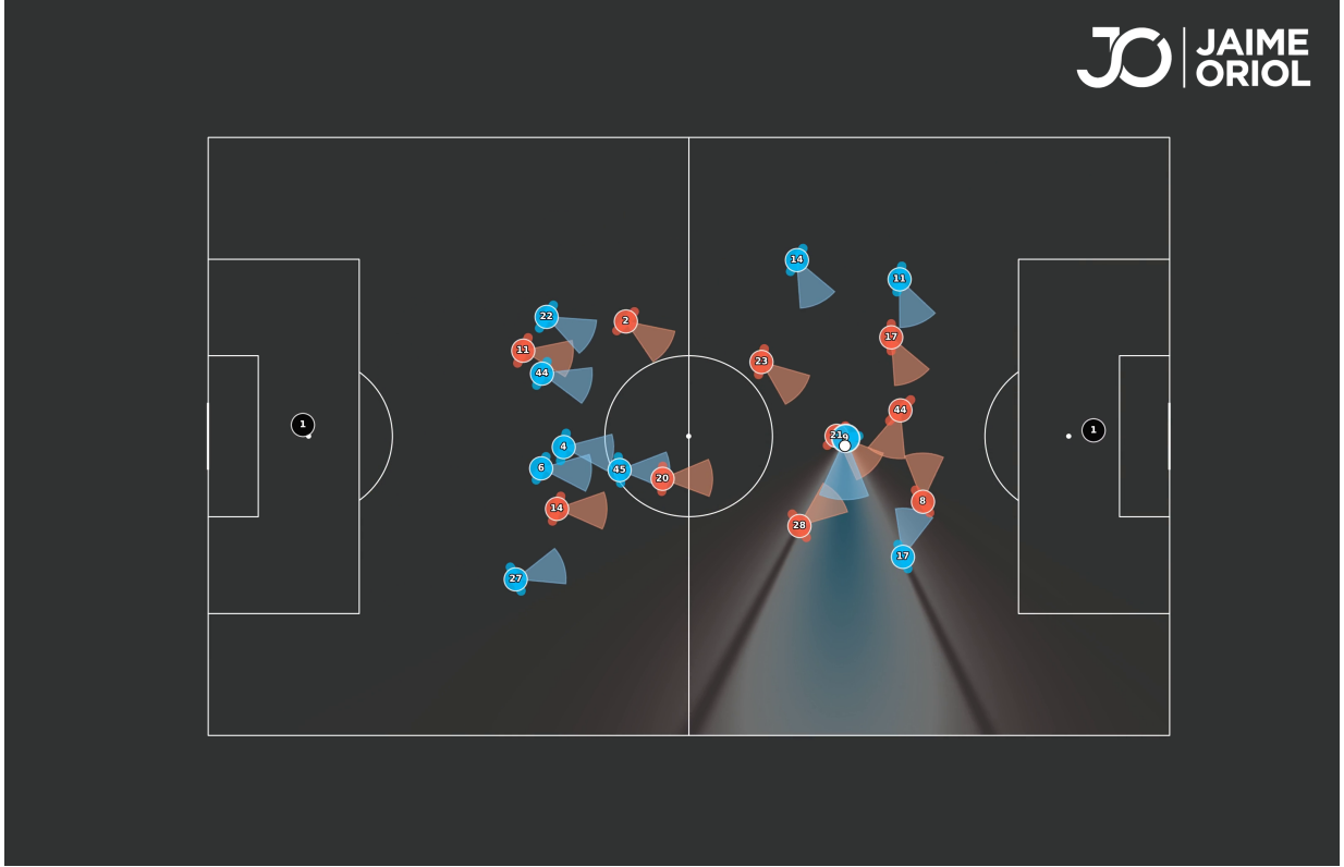
Figure 4: Vision model. Per-player field of view: a 120^\circ probabilistic cone around the measured head yaw, with speed-dependent radial and angular decay, plus torso occlusion computed from the real shoulder width of every occluder. Frame from the A. Knauff sequence (Frankfurt–Union). Video: Vision_Video.mp4 .
