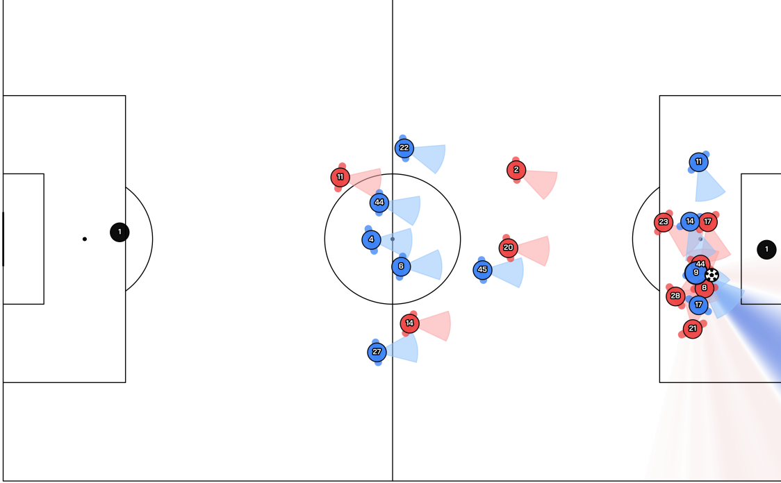
Figure 5: Vision model. Per-player field of view: a 120^\circ probabilistic cone around the measured head yaw, with speed-dependent radial and angular decay, plus torso occlusion computed from the real shoulder width of every occluder. Frame from the A. Knauff sequence (Frankfurt–Union). Video: Vision_Video.mp4 .
