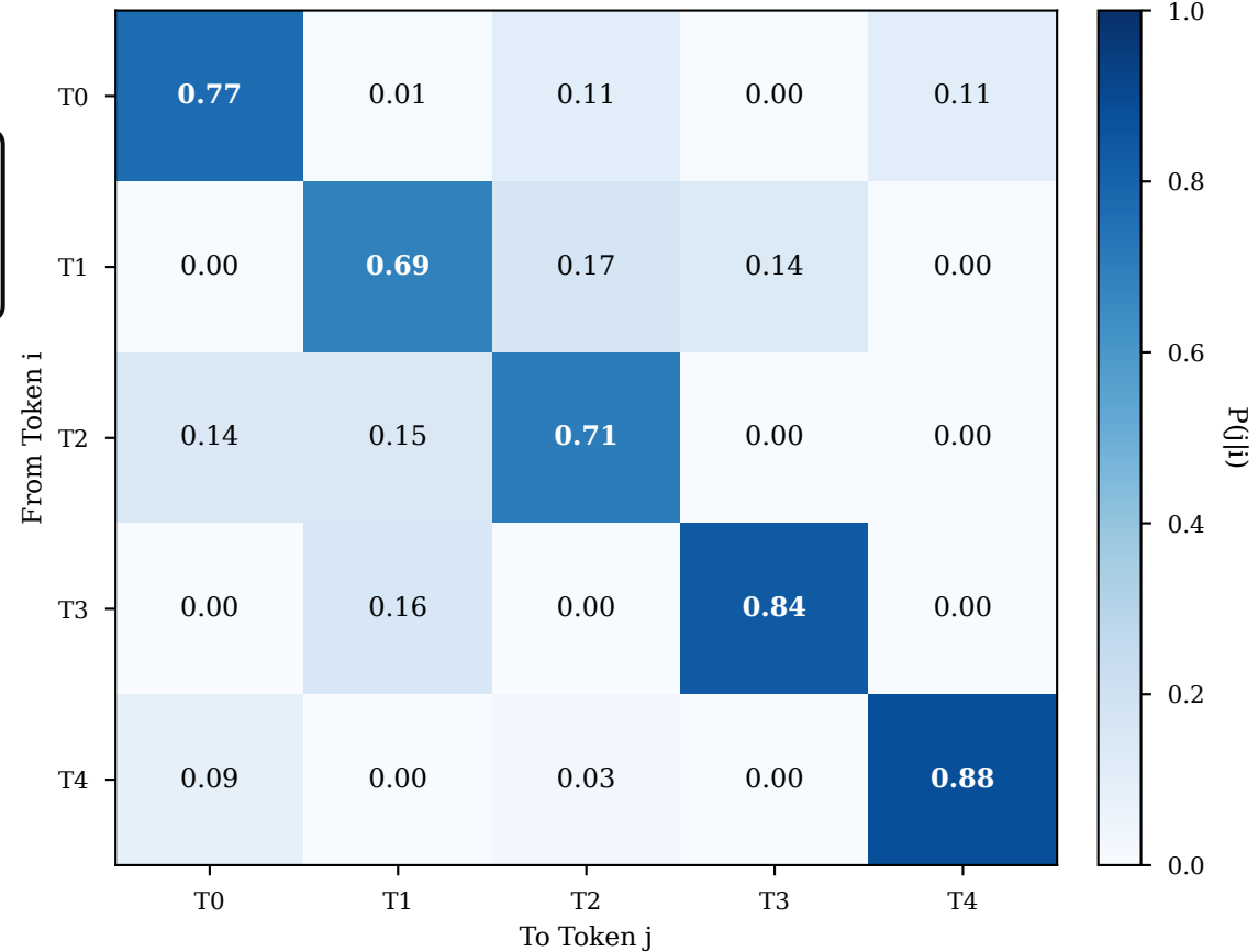
Transition Matrix A | Diag mean=0.78
