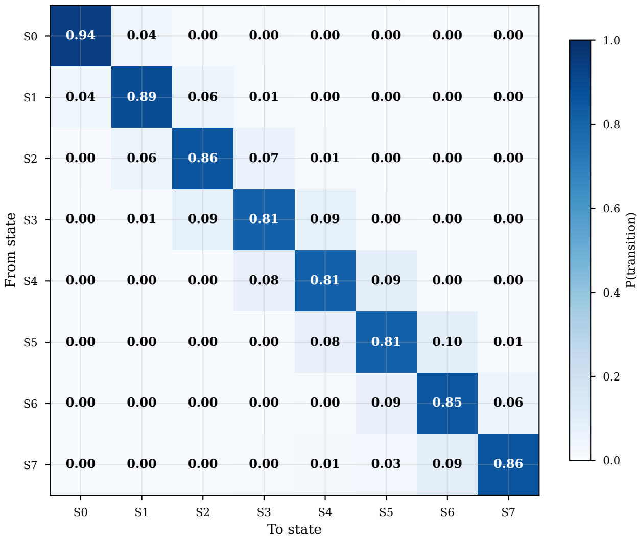
Transition Matrix A (Weather, K=8)
