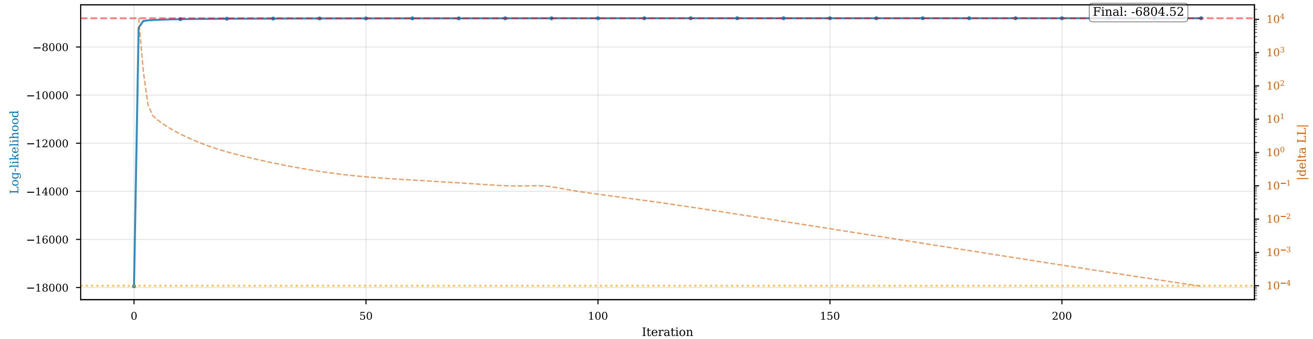
Baum-Welch ETTh2 | Iters=231, Final LL=-6804.52
