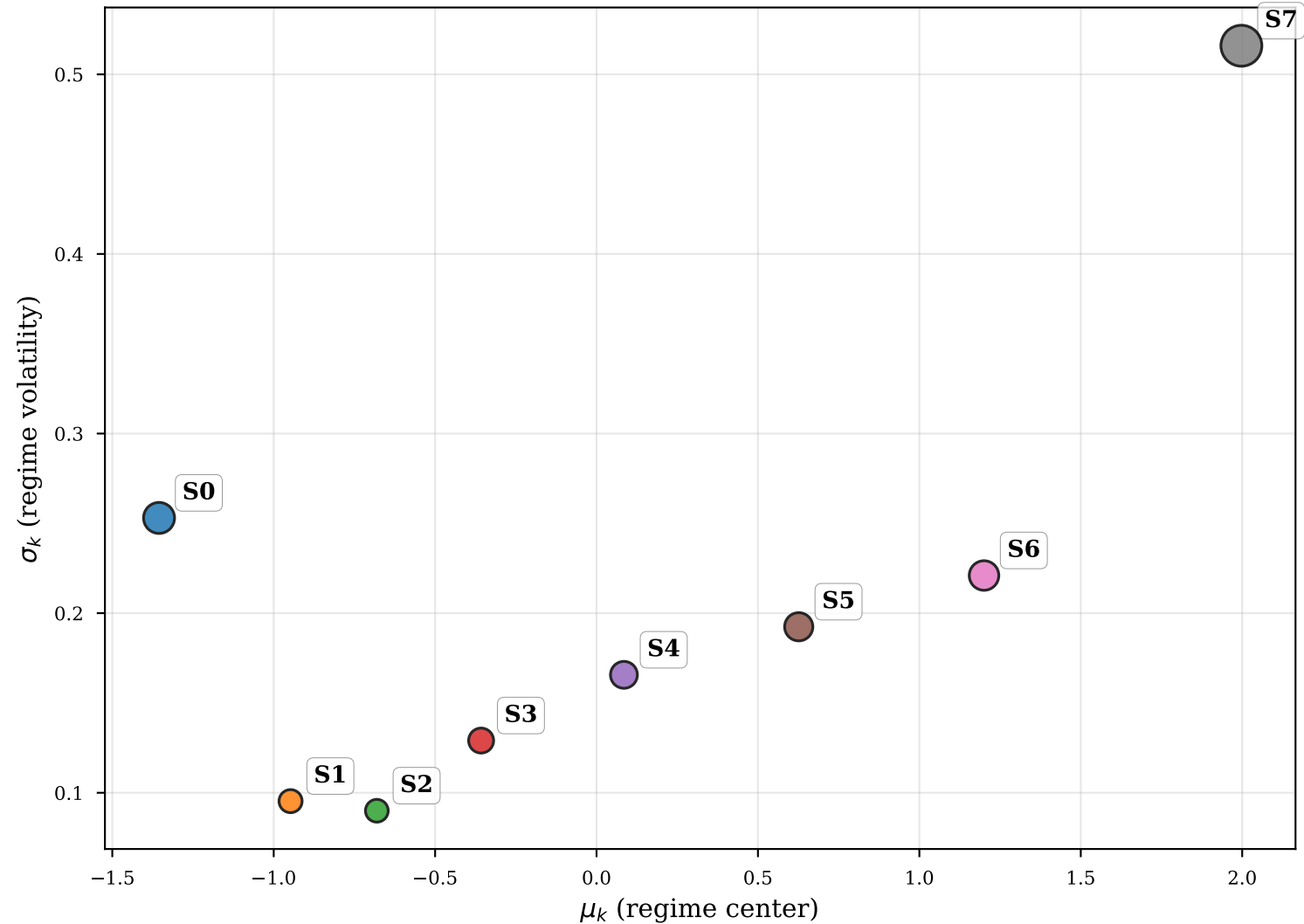
Embedding Space: HMM States (Weather, K=8)
