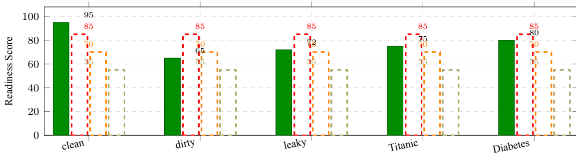
Figure 2: Readiness scores across five datasets. Dashed lines indicate grade thresholds ( A \geq 85 , B \geq 70 , C \geq 55 ).
