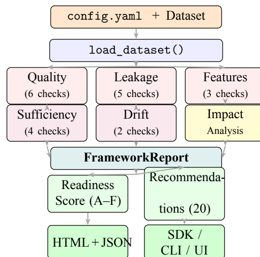
Figure 1. ml-framework analysis pipeline. A dataset and a configuration file flow through six parallel analysis phases, are aggregated into a FrameworkReport , scored (0–100, grade A–F), and exported as HTML, JSON, or via Python SDK.
