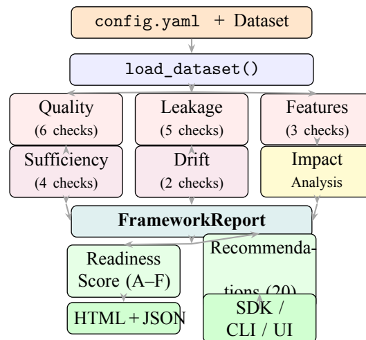
Figure 1. ml-framework analysis pipeline. A dataset and a configuration file flow through six parallel analysis phases, are aggregated into a FrameworkReport , scored (0–100, grade A–F), and exported as HTML, JSON, or via Python SDK.
