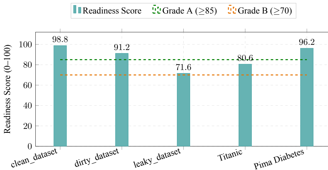
Figure 4.1. Readiness scores across five principal datasets. The clean control scores highest; only the two datasets with confirmed target leakage are downgraded to grade B.
