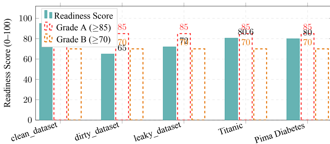
Figure 3.1. Readiness scores across five principal datasets. The clean control achieves grade A; leaky and dirty datasets are appropriately downgraded.
