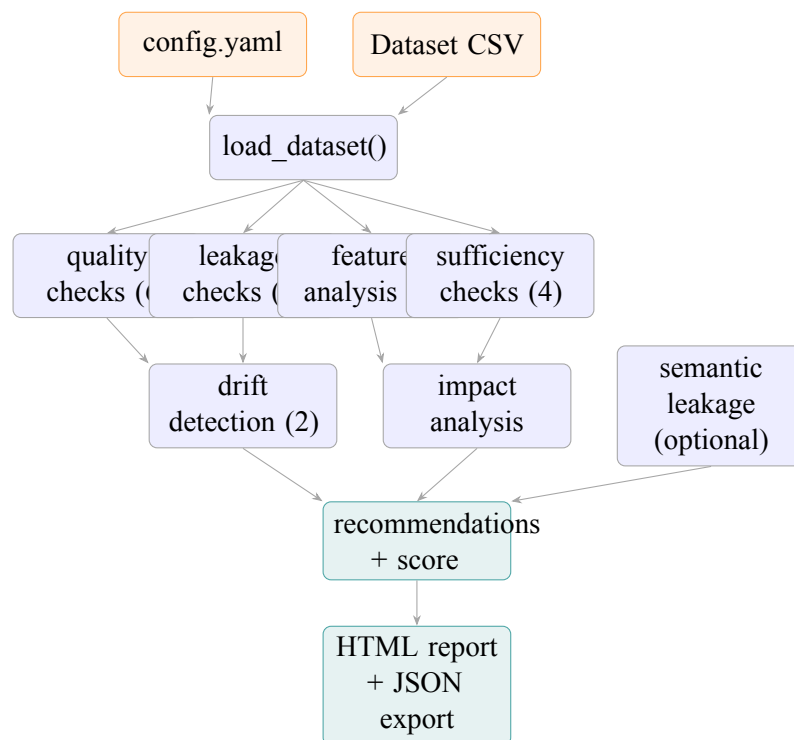
Figure 2.1. ml-framework pipeline. Arrows show data flow from configuration and dataset through six parallel analysis modules to recommendations, readiness score, and reports.
