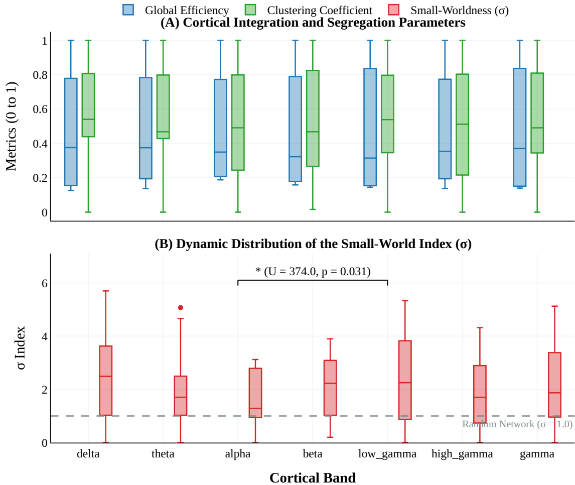
Figure 7 – Topological Dynamics and Small-World Optimization in the Visual Cortex. (A) High temporal variability of Global Efficiency and Clustering Coefficient. The substantial dispersion (ranging from 0.2 to 0.8) illustrates the volatile dynamics of cortical processing, as the network continuously balances moments of strong local processing (high clustering) with global communication jumps (high efficiency). (B) Comparison of the Small-World Index ( \sigma ) between the Alpha (8-12 Hz) and Low-Gamma (30-59 Hz) bands. The asterisk (*) denotes a statistically significant increase in Small-World topology during Low-Gamma. The pronounced dispersion (elongated whiskers) underscores that the network operates through transient, high-efficiency topological pulses rather than remaining in a static optimized configuration.
