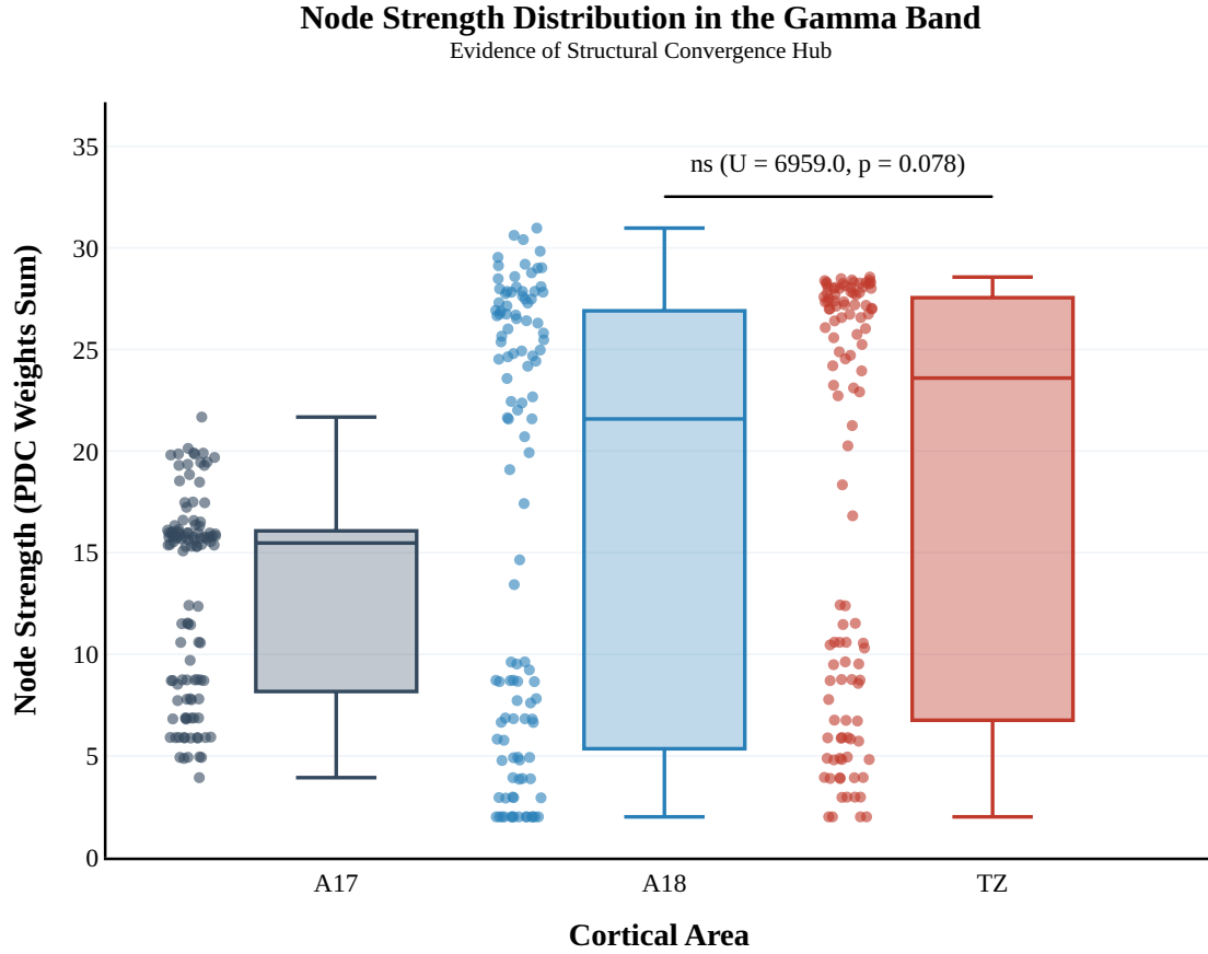
Figure 8 – Node Strength Distribution in the Gamma Band. Area 17 displays restricted centrality with low variability. In contrast, both the Transition Zone (TZ) and Area 18 exhibit bimodal distributions with high variability. The Transition Zone operates under a connectivity load tendentially superior to that of Area 18, highlighting its role as a primary interhemispheric convergence hub.
