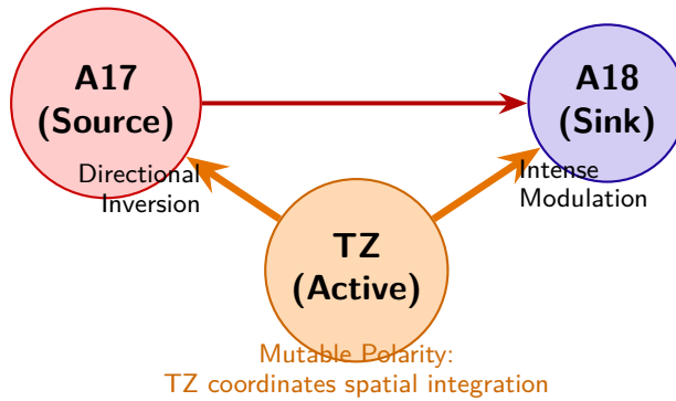
Figure 6 – Evolutionary Topological Mapping of Information Net-Flow (Low-Gamma Band) . In-degree minus out-degree proportions. (A) During the baseline period, the network operates in a strict predictive visual hierarchy, where Area 17 (A17) is the primary driving pole and Area 18 (A18) the passive sink, with the Transition Zone (TZ) in a neutral state. (B) At the exact moment of the stimulus (moving grating onset), the topology undergoes active remodeling. The TZ reverses its passive polarity and adopts acute modulation dynamics, drastically altering the edge weights (arrow thickness) and proving that mesoscopic flexibility reacts transiently to the peripheral stimulus input.
