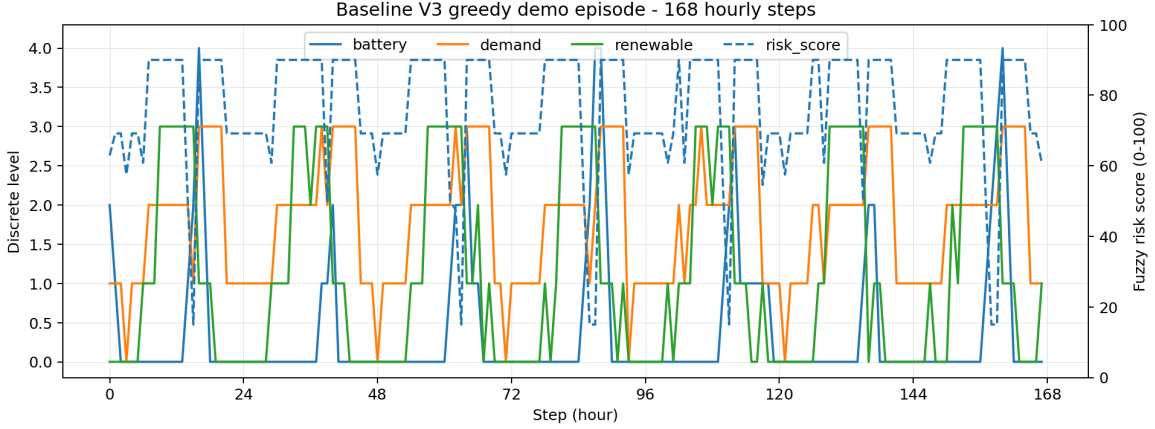
Figure 5: Temporal evolution of the baseline V3 greedy demo episode. The figure illustrates how demand, renewable availability, battery state and fuzzy risk vary across the 168-hour synthetic week. The left axis uses discrete state levels, while the right axis uses the fuzzy risk scale from 0 to 100.
