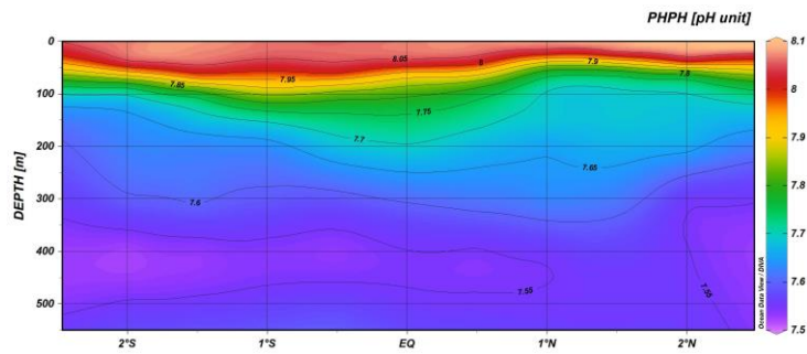
Figure 18 : section 23 W, pHt (@25°C), PIRATA FR35
