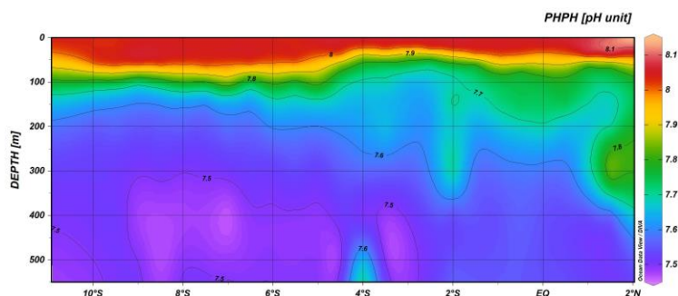
Figure 17 : section 10 W, pHt (@25°C), PIRATA FR35
