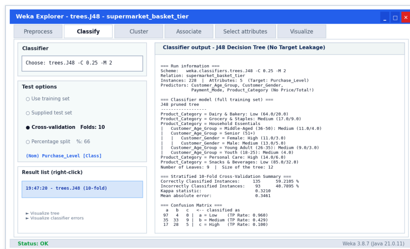
Figure 9.2: Weka Classify Tab: J48 Decision Tree Model Execution & 10-Fold Cross-Validation Console Output
