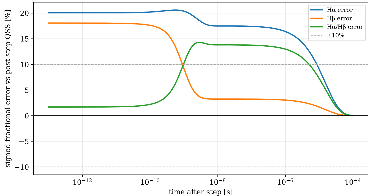
Balmer transient errors: Te 2.95→3.24 eV, ne=1.39e+14 cm -3
