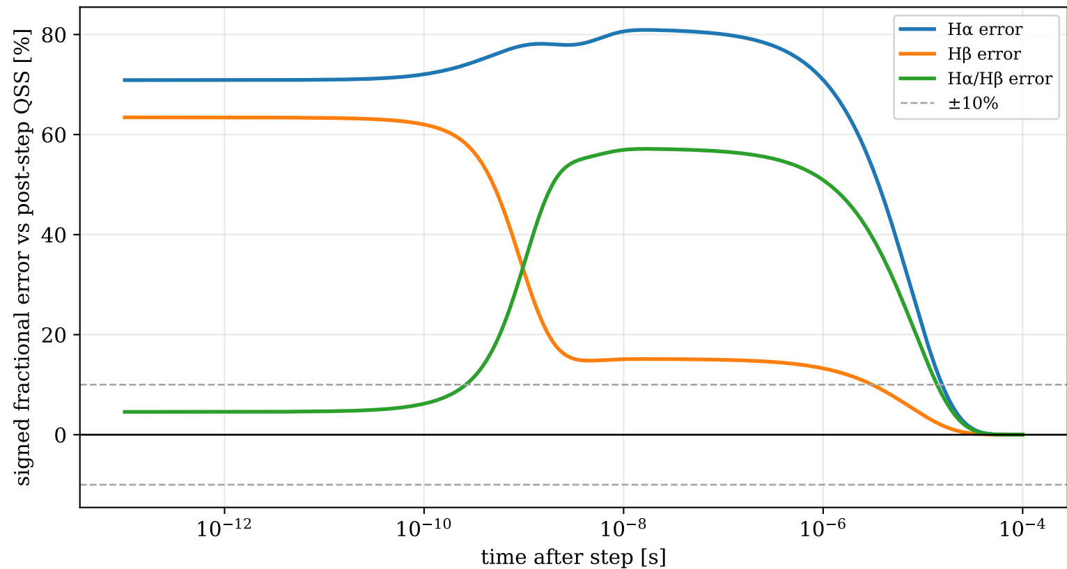
Balmer transient errors: Te 2.95→3.91 eV, ne=1.39e+14 cm -3
