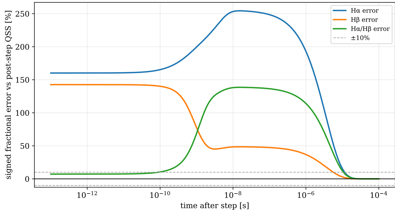
Balmer transient errors: Te 2.95→4.94 eV, ne=1.39e+14 cm -3
