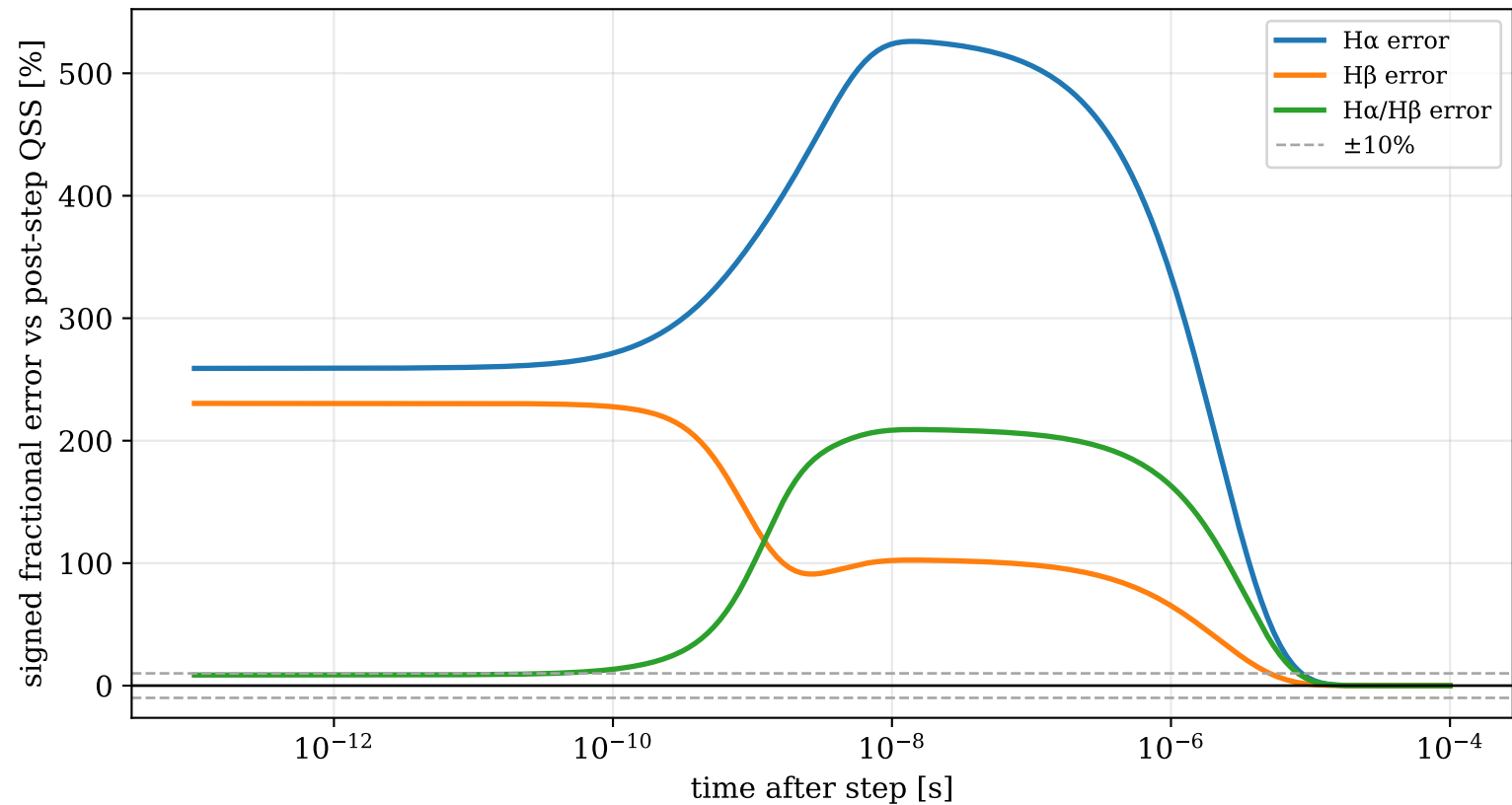
Balmer transient errors: Te 2.95→5.96 eV, ne=1.39e+14 cm -3
