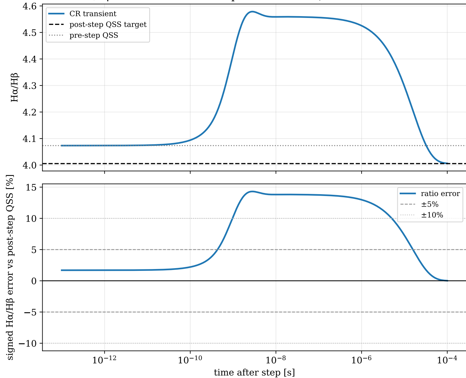
H \alpha /H \beta transient after Te step: 2.95→3.24 eV, ne=1.39e+14 cm -3
