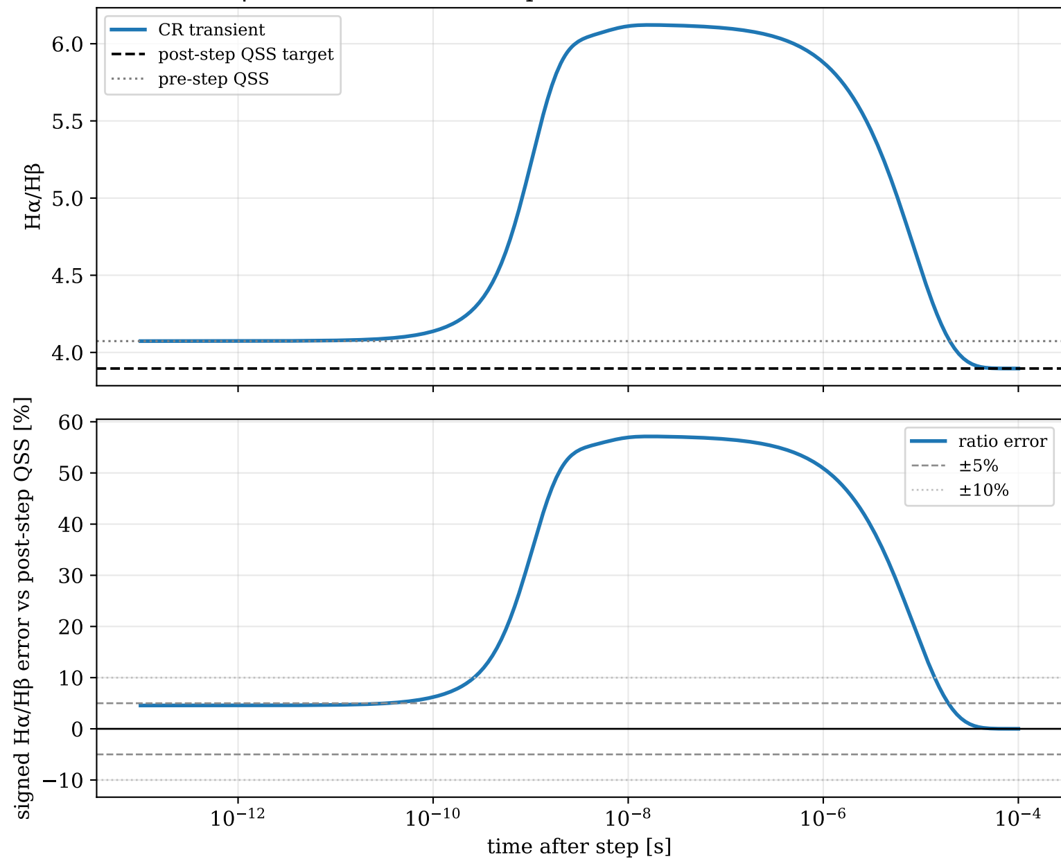
H \alpha /H \beta transient after Te step: 2.95→3.91 eV, ne=1.39e+14 cm -3
