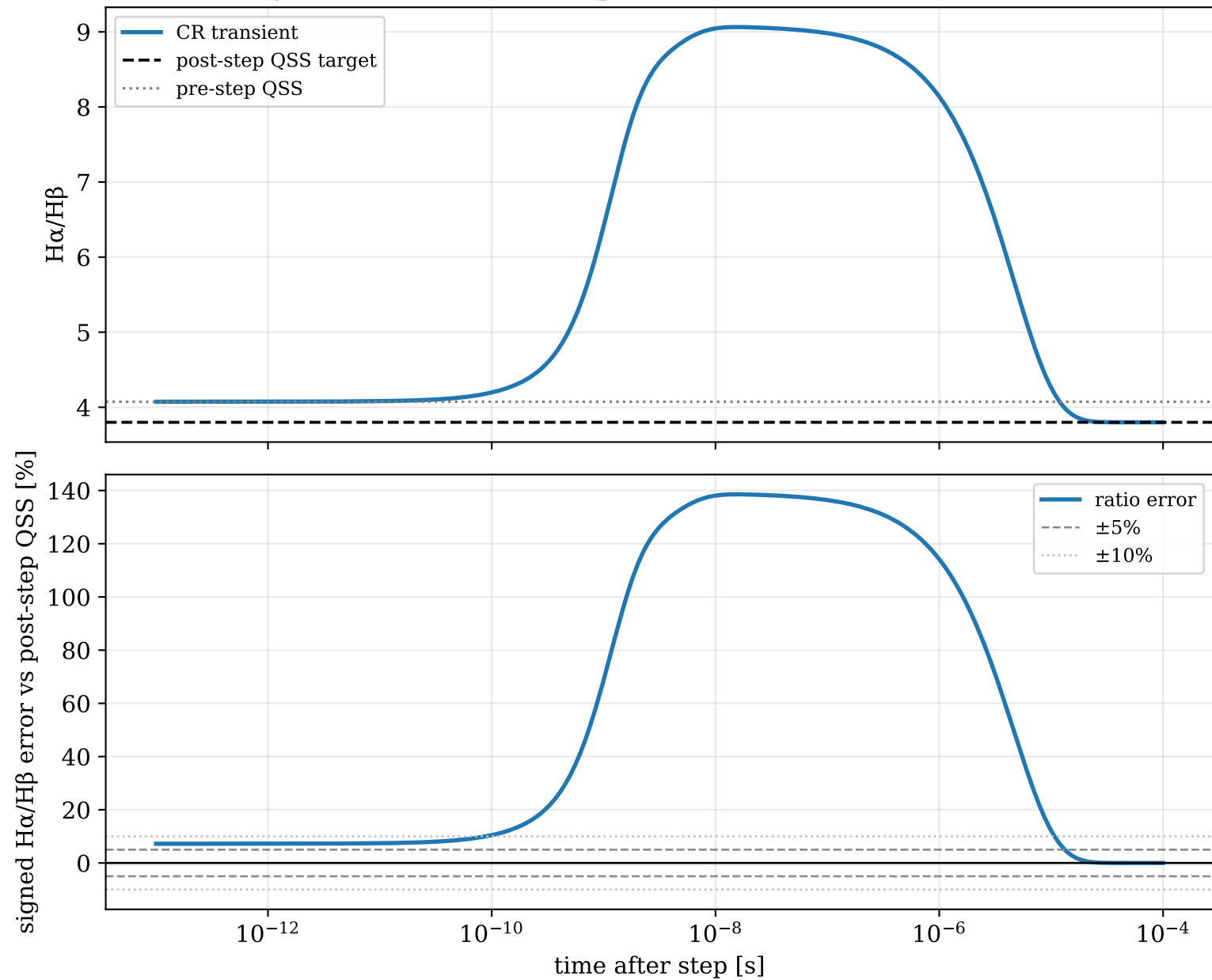
H \alpha /H \beta transient after Te step: 2.95→4.94 eV, ne=1.39e+14 cm -3
