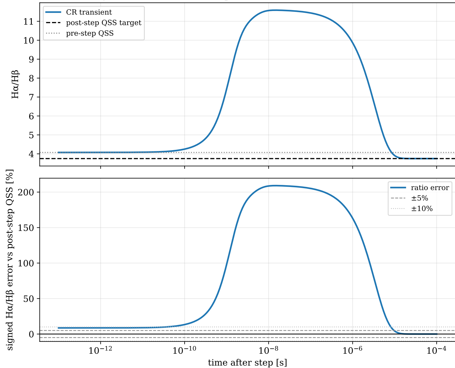
H \alpha /H \beta transient after Te step: 2.95→5.96 eV, ne=1.39e+14 cm -3
