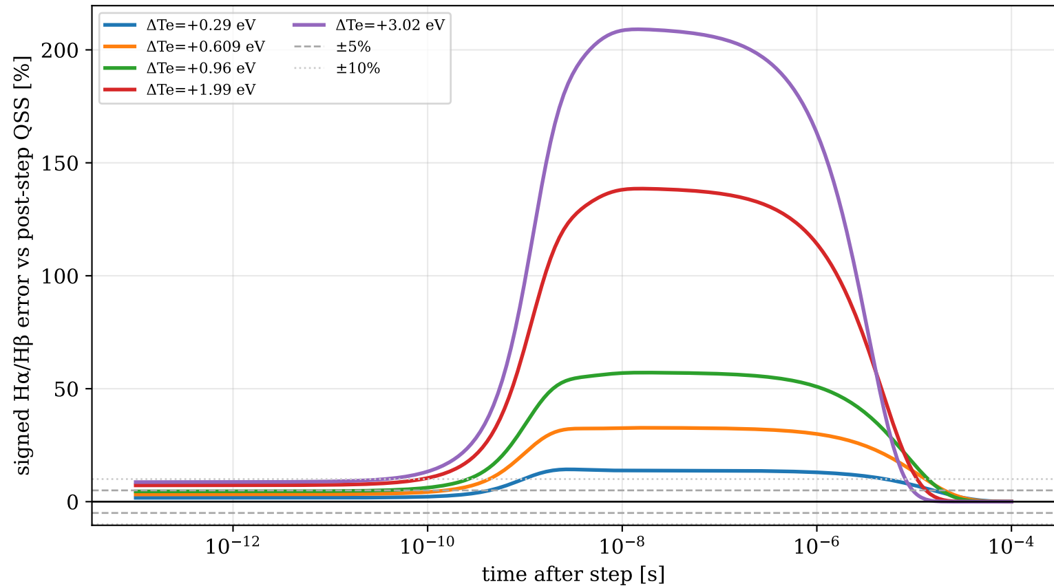
\text{H}\alpha/\text{H}\beta transient ratio error at n_e=1.39\text{e}+14\text{ cm}^{-3}
