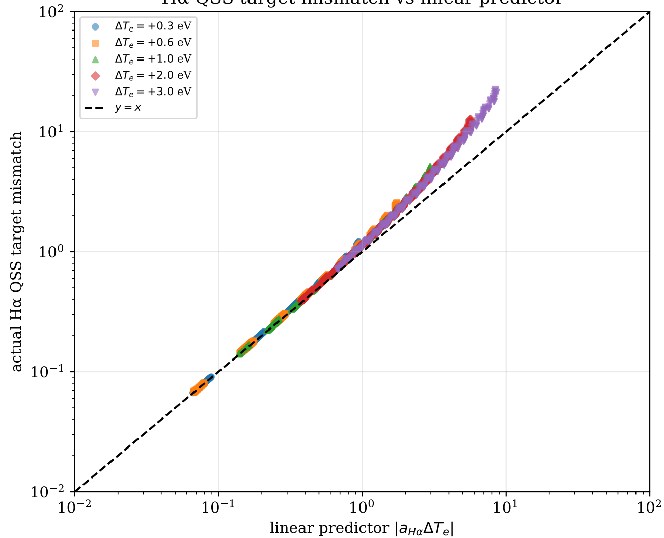
H \alpha QSS target mismatch vs linear predictor
