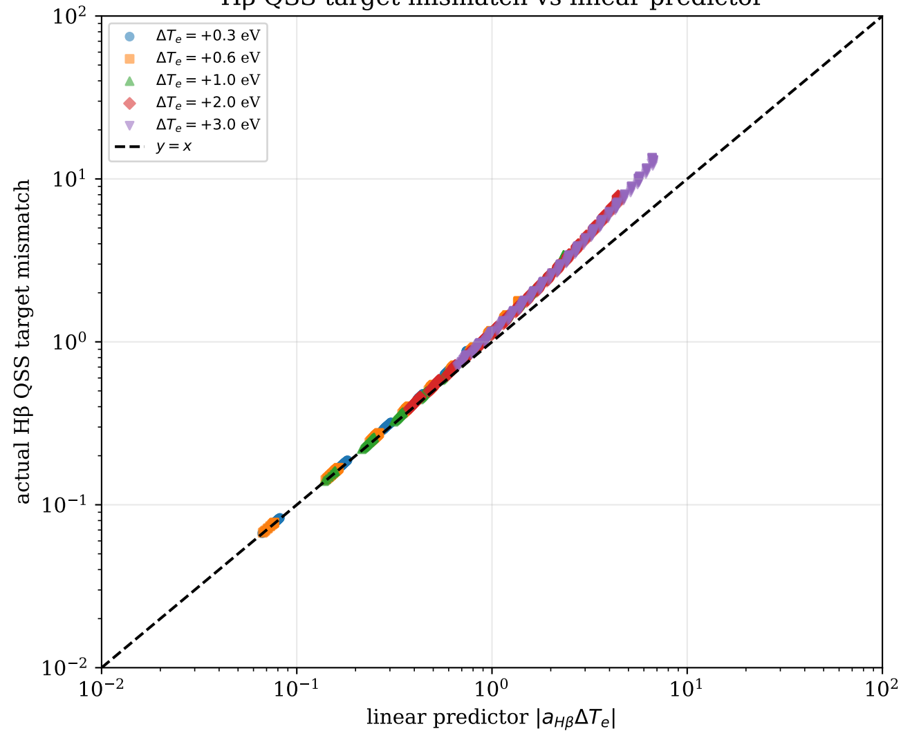
H \beta QSS target mismatch vs linear predictor
