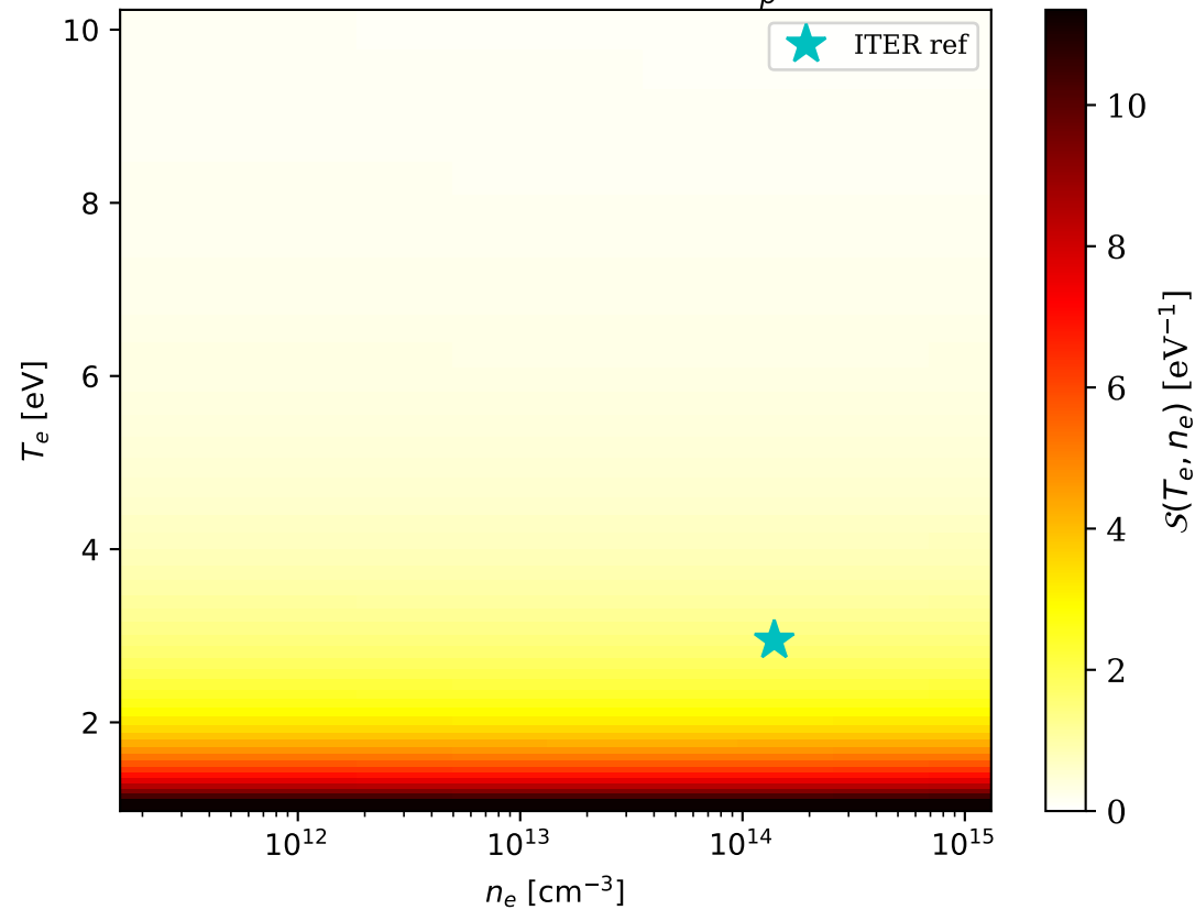
(a) QSS manifold sensitivity \mathcal{S} = \max_p |\partial_{T_e} \ln r_p^{\text{QSS}}|
