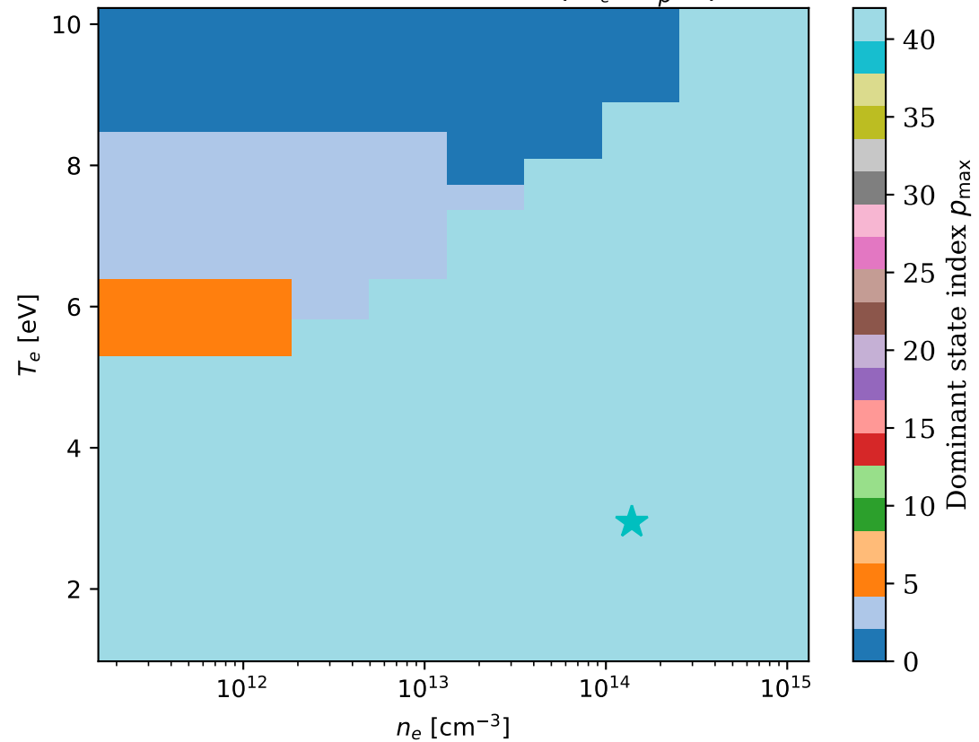
(b) State p maximising |\partial_{T_e} \ln r_p^{\text{QSS}}|
