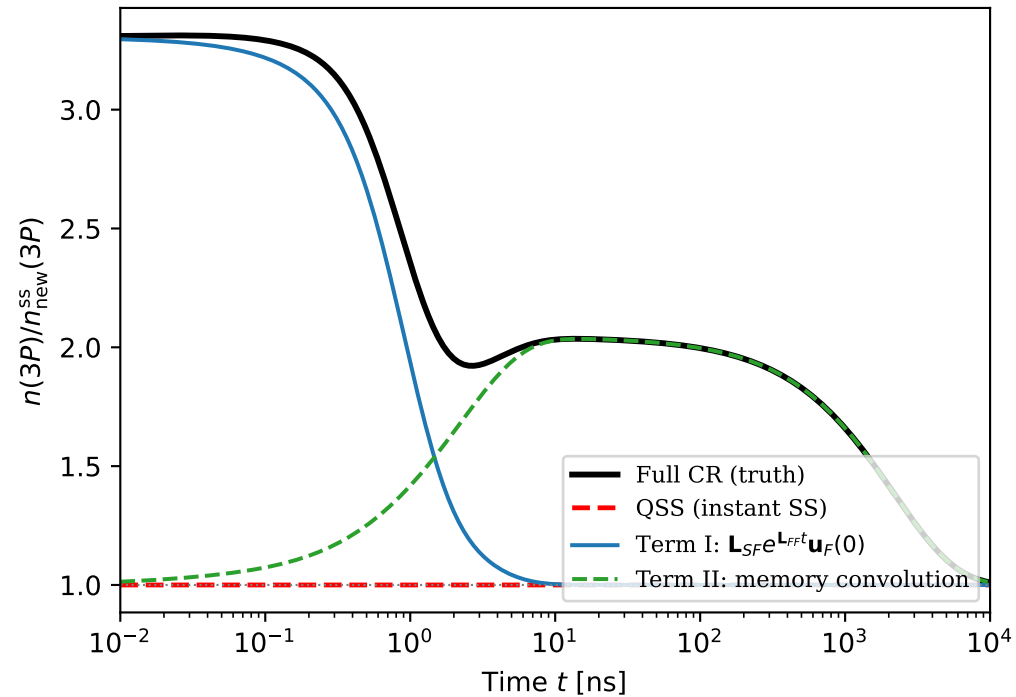
(a) n(3P) transient: MZ decomposition T_e step 3.0 \rightarrow 6.0 eV, n_e = 10^{14} cm ^{-3}
