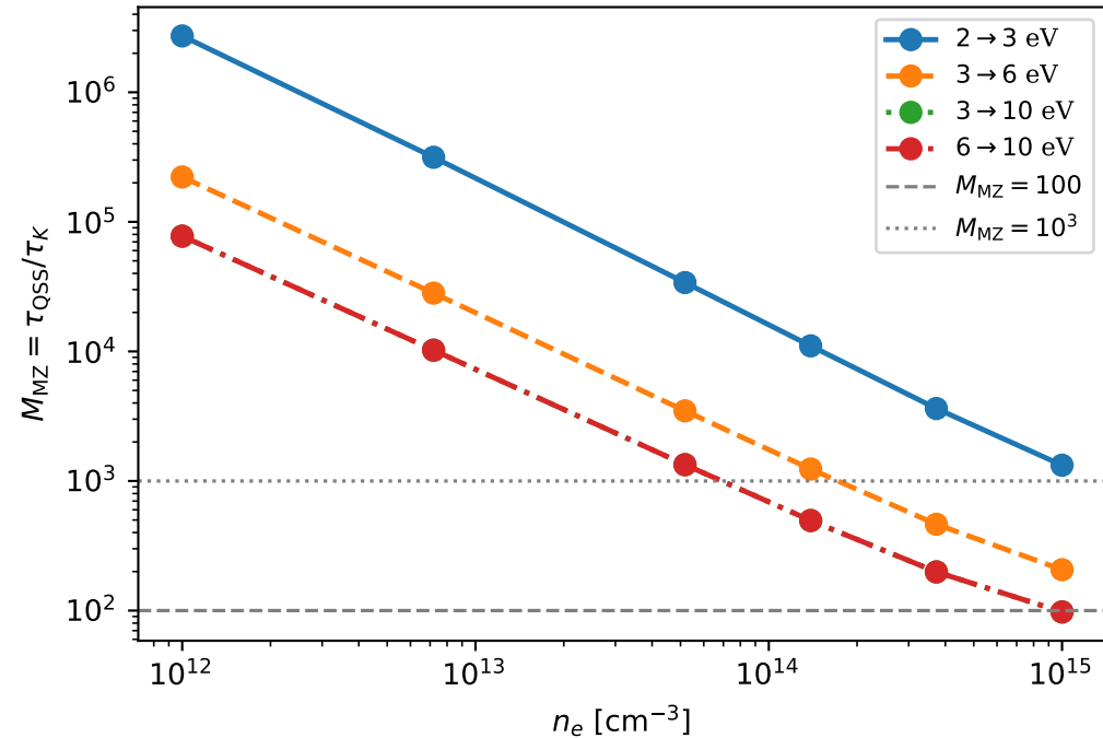
(b) Term~II suppression: M_{MZ} \gg 1 (Term~II \leq M_{MZ}^{-1} \times Term~I)
