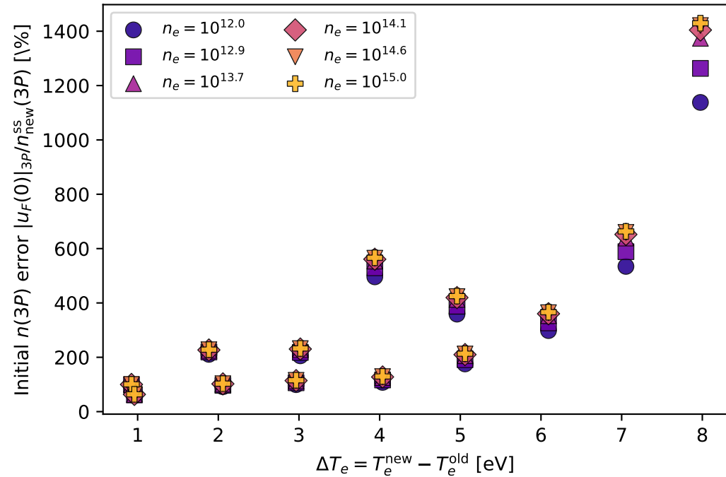
(a) Term~I amplitude: initial fast-state mismatch (sets QSS error magnitude)
