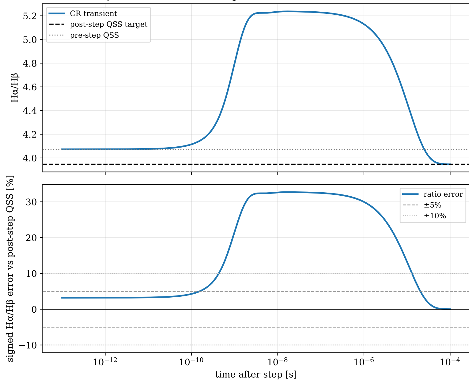
H \alpha /H \beta transient after Te step: 2.95→3.56 eV, ne=1.39e+14 cm -3
