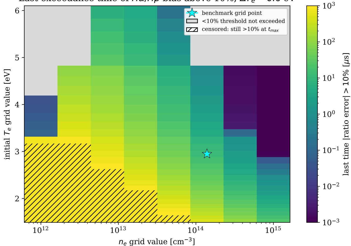
Last exceedance time of H\alpha/H\beta bias above 10%, \Delta T_e \approx 0.6 eV
