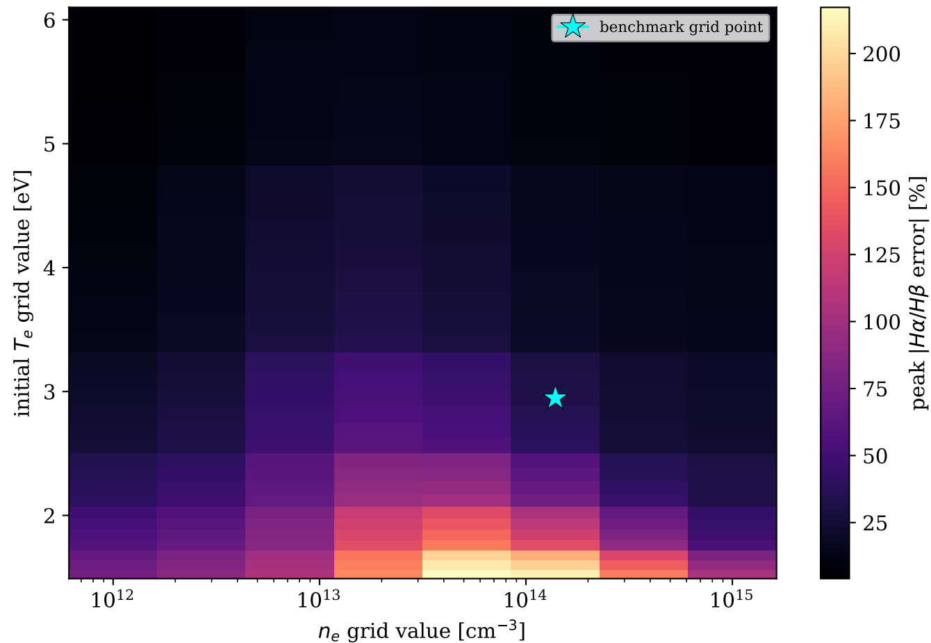
Peak transient H\alpha/H\beta ratio error, \Delta T_e \approx 0.6 eV
