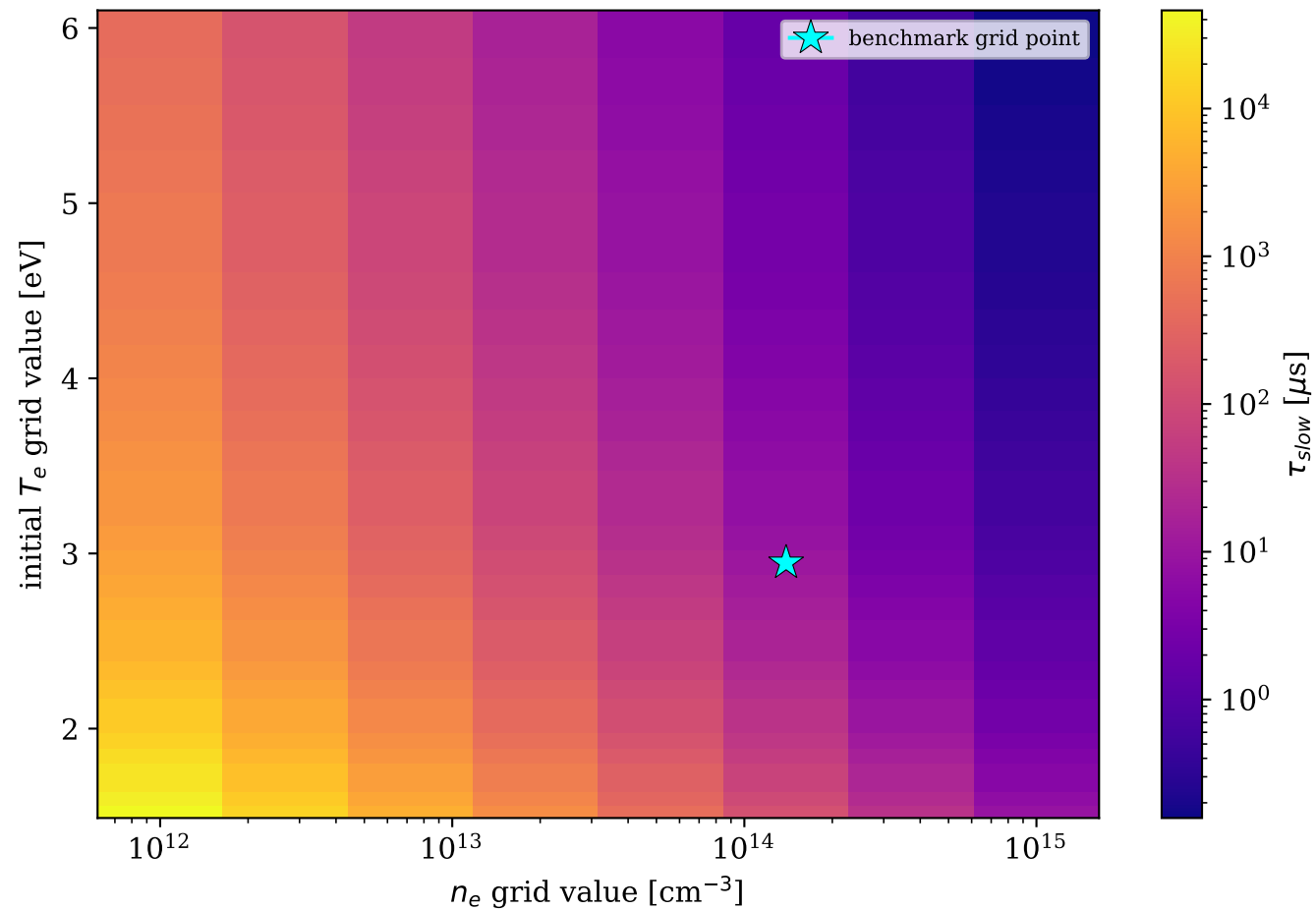
Slow CR decay time after step, \Delta T_e \approx 0.6 eV
