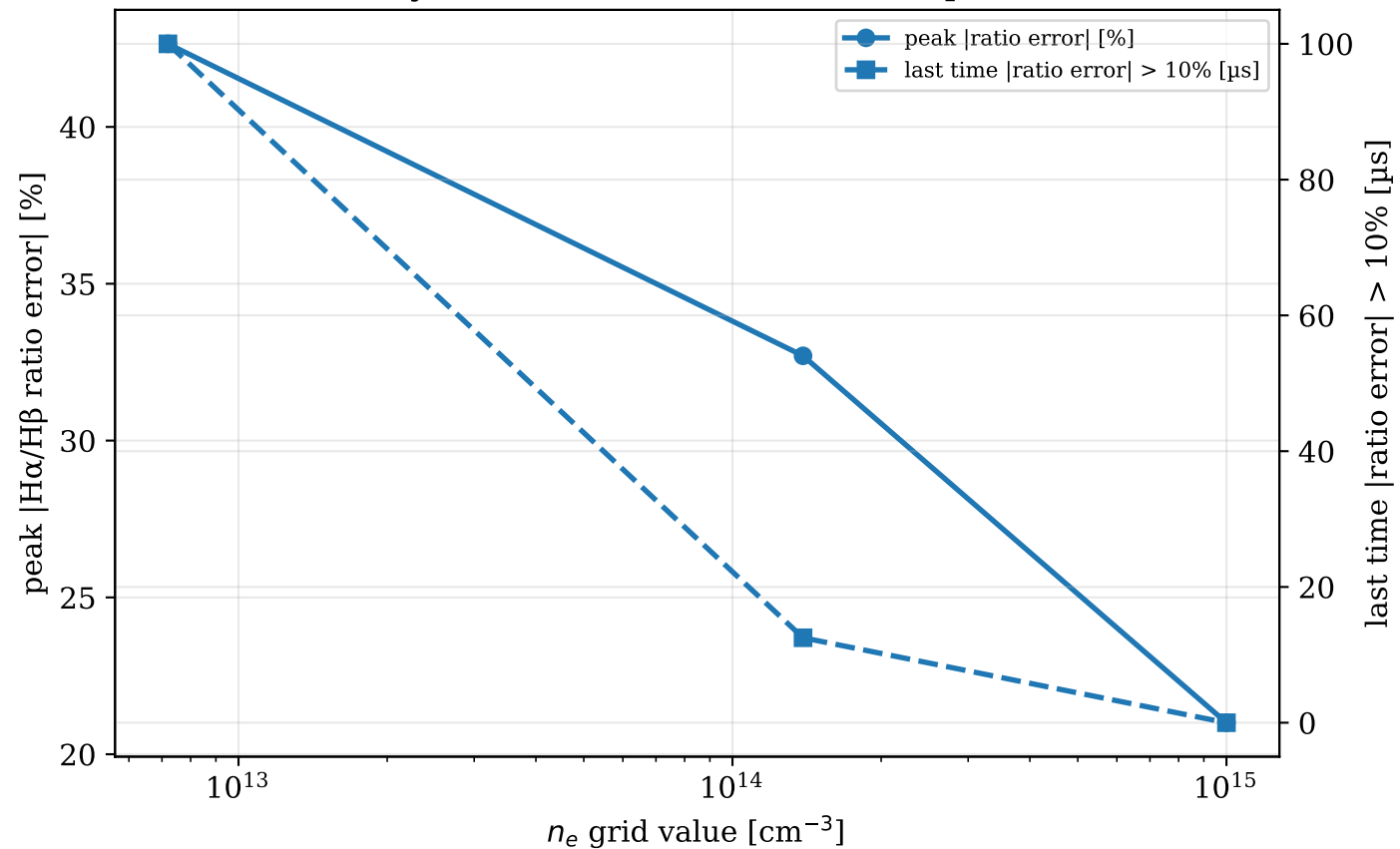
Density robustness at reference temperature
