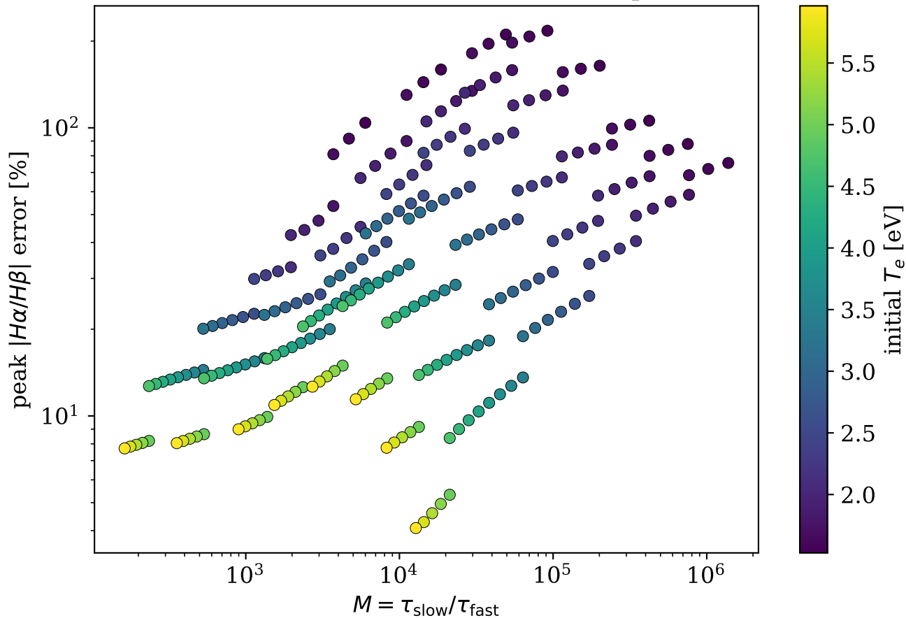
Peak Balmer-ratio bias vs timescale separation
