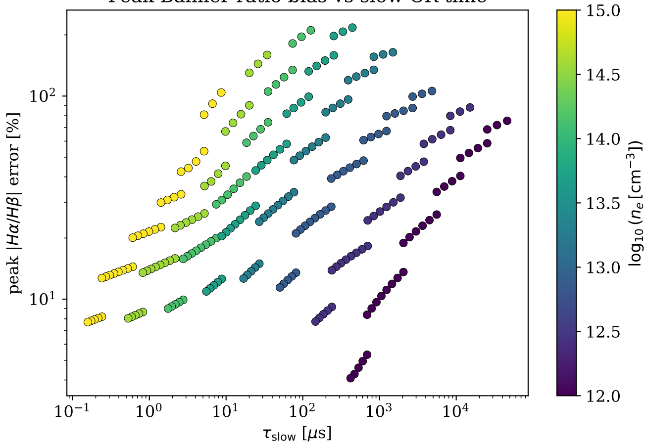
Peak Balmer-ratio bias vs slow CR time
