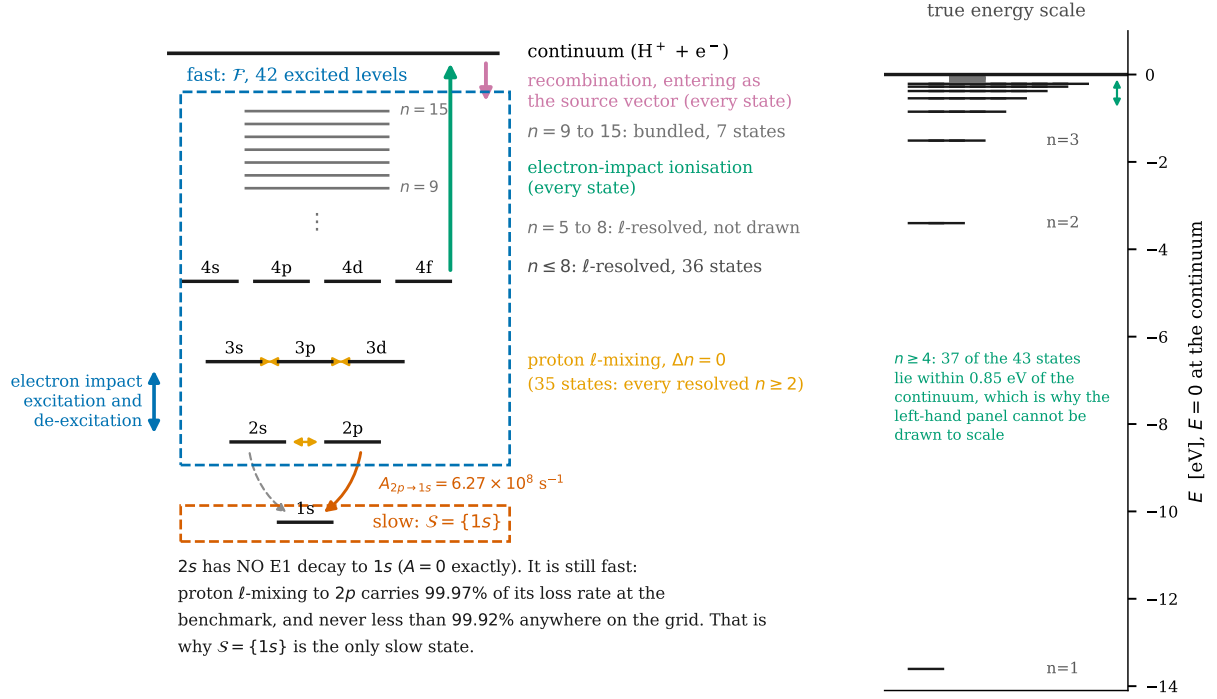
Figure 2.1: The 43-state space and the five processes the rate matrix contains. Left: the level structure. Hydrogen is \ell -resolved up to n = 8 , which is 36 states, and bundled into one level per n from n = 9 to 15, which is 7 more. Vertical spacing is schematic; the right-hand panel gives the true energies, and shows why, with 37 of the 43 states lying within 0.85 eV of the continuum, a to-scale ladder would be unreadable. Five processes appear in the matrix: electron-impact excitation and de-excitation between levels, radiative decay ( A_{2p \rightarrow 1s} = 6.27 \times 10^8 \text{ s}^{-1} , and 34 of the 36 resolved states carry a non-zero decay rate), electron-impact ionisation from every state, recombination, which enters as the source vector rather than as a matrix element and feeds every state, and proton-impact \ell -mixing, which is \Delta n = 0 and acts on 35 states, every resolved level with n \geq 2 . Only the n = 2 and n = 3 mixing arrows are drawn; at n = 4 the sublevels are too close together for an arrow to render legibly. The dashed boxes mark the partition the analysis rests on, and 2s is why it can be drawn where it is. 2s has no E1 decay to the ground state, its radiative rate to 1s being exactly zero in the matrix, so on radiative grounds alone it would be metastable and would belong with the slow states. It is nonetheless fast, because proton \ell -mixing to 2p carries 99.97% of its total loss rate of 1.47 \times 10^{11} \text{ s}^{-1} at the benchmark, and never less than 99.92% anywhere on the grid, rising to 99.99% at the cold edge. That single channel is what leaves \mathcal{S} = \{1s\} as the only slow state and the remaining 42 levels in the fast manifold. The state list, including which levels are bundled and every ionisation energy, is read from the model's own state index, not written into this figure.
