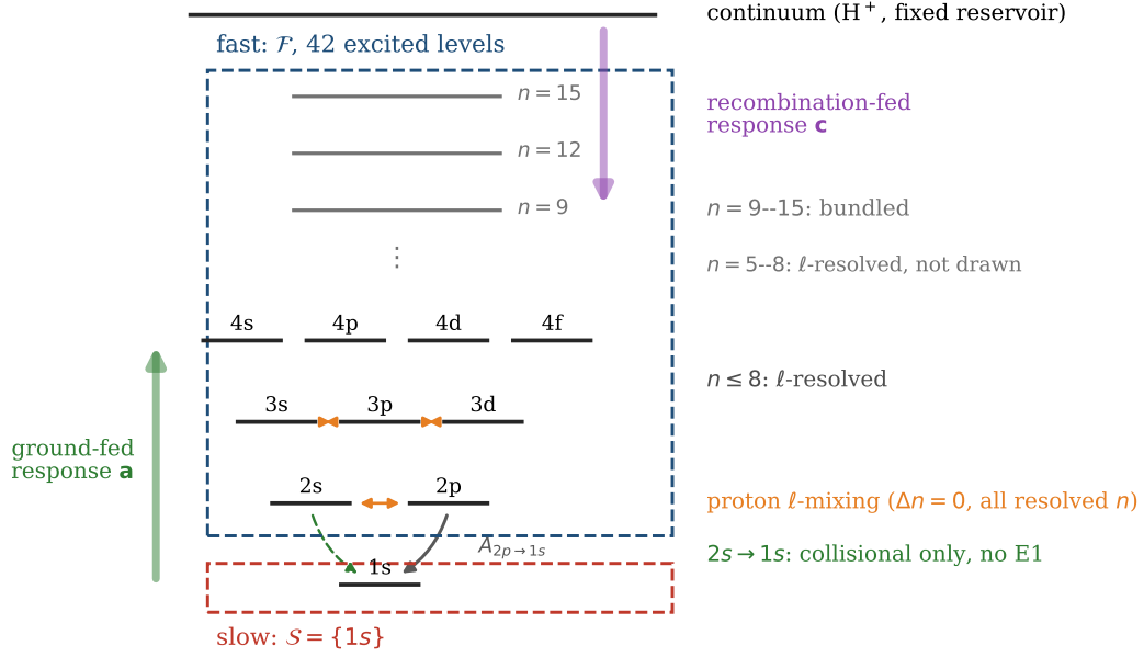
Figure 3.1: The collisional–radiative network of atomic hydrogen and the partition used in Section 3.4. Levels with n \leq 8 are resolved in orbital angular momentum; n = 9–15 are bundled with a statistical \ell -distribution. Proton-impact \ell -mixing (orange) couples sublevels within every resolved shell and is the dominant loss channel for the metastable 2s level, which has no electric-dipole route to the ground state; arrows are drawn for n = 2 and n = 3 only, the n = 4 sublevels being too closely spaced on this schematic for a legible arrow. The broad arrows are not elementary transitions: \mathbf{a} = -\mathbf{L}_{FF}^{-1}\mathbf{L}_{FS} and \mathbf{c} = -\mathbf{L}_{FF}^{-1}\mathbf{S}_F are network responses , each summing every cascade route from its reservoir into a given level (Section 3.5.3). Vertical spacing is schematic and not drawn to energy scale.
