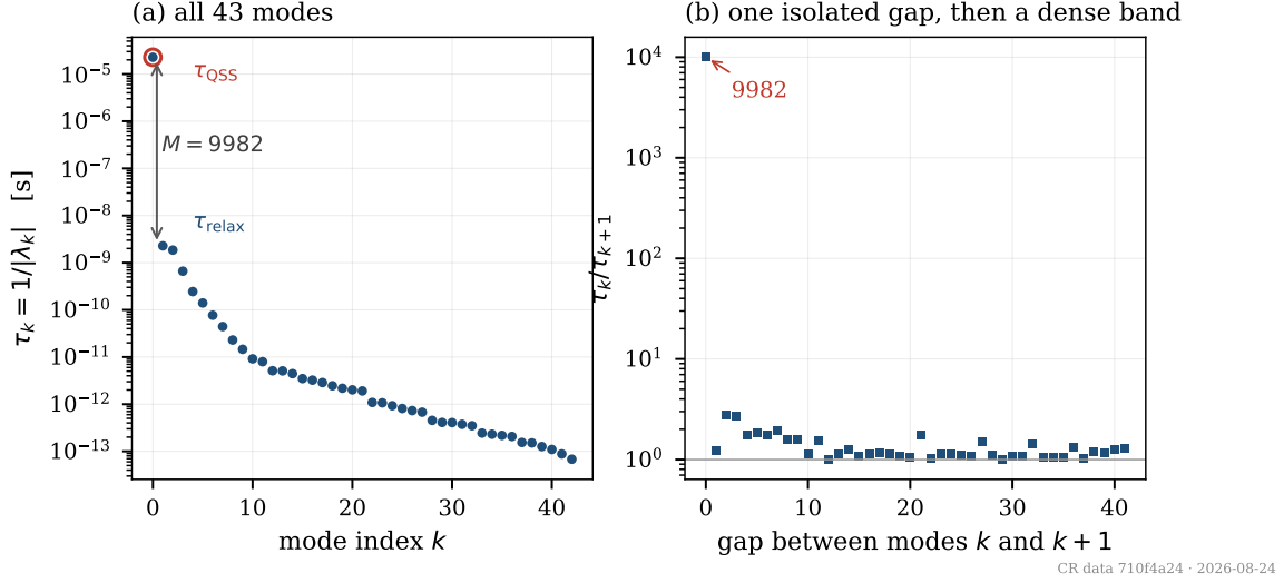
Figure 3.2: Relaxation timescales at the benchmark point. (a) All 43 modes. The slowest, \tau_{\text{QSS}} , is the relaxation of the ground-state population; the next, \tau_{\text{relax}} , is the slowest-decaying mode of the excited manifold, the bottleneck of the fast set, and their ratio is the separation M . (b) The ratio of consecutive timescales, which shows that the first gap is exceptional: the largest of the other 41 is 2.80, so the first exceeds every competitor by a factor of 3567 and the 42 fast modes form a dense band rather than a hierarchy.
